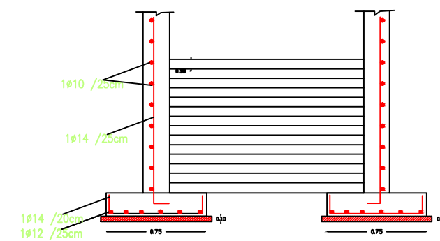
sec 1-1
