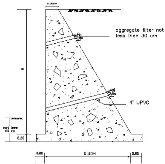
MASONRY RETAINING WALL - TYPICAL SEC.
