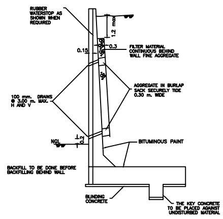
TYPICAL SECTION IN L-SHAPED RETAINING WALL
