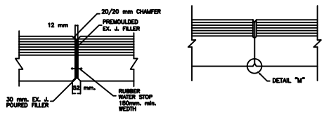
EXPANSION JOINT PLAN
