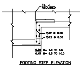
FOOTING STEP ELEVATION
