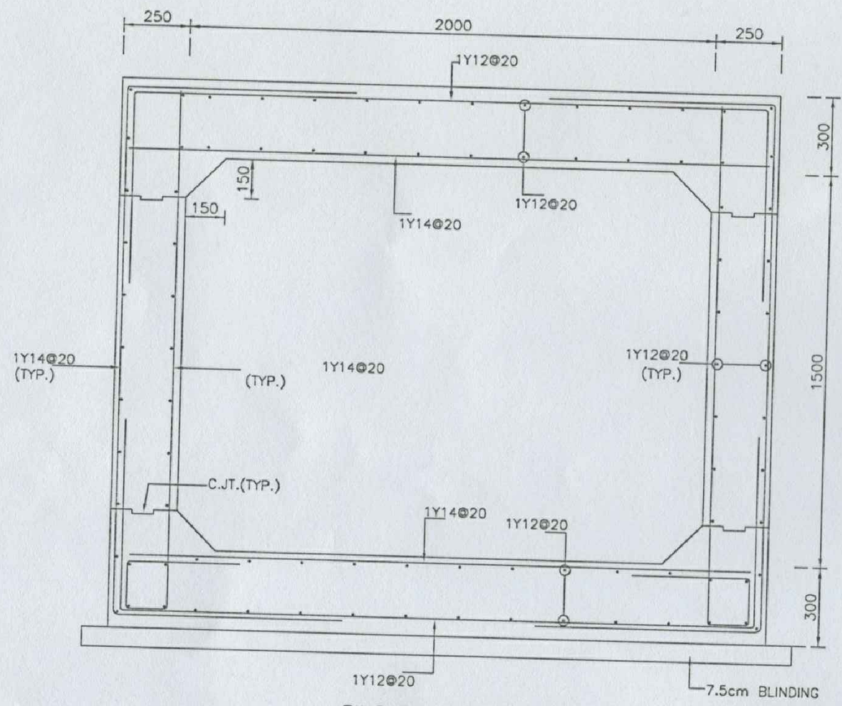
SINGLE CELL BOX CULVERT TYPICAL SECTION
