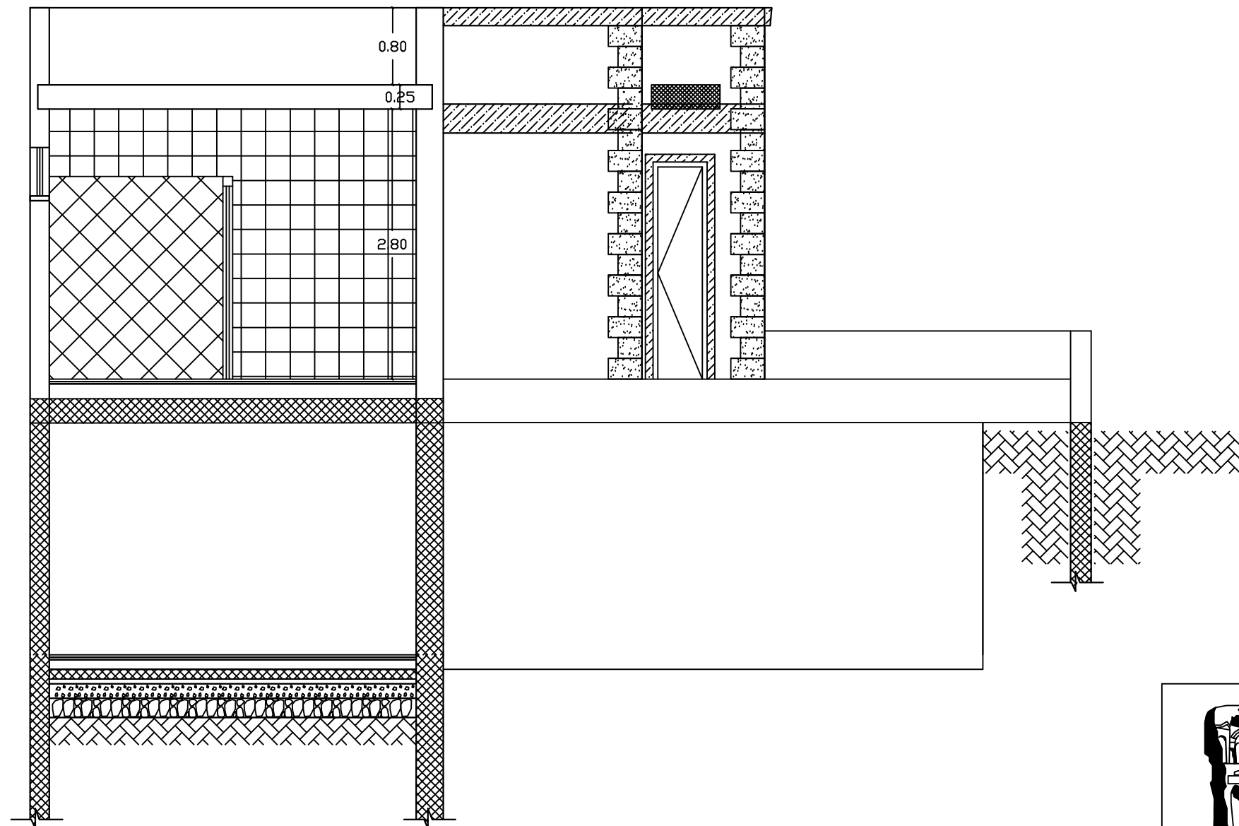
SECTION B-B
