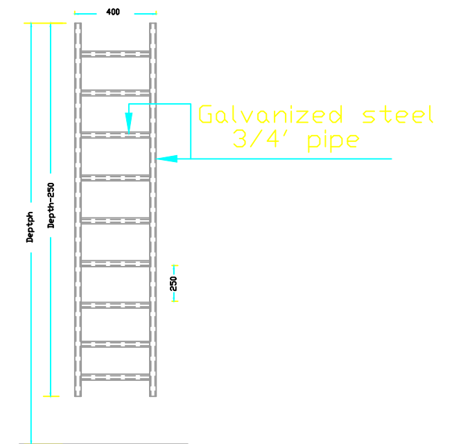
THE INSIDE STEEL STAIR DETAIL
