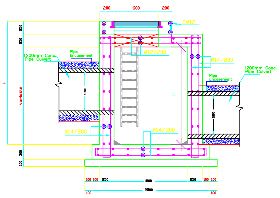
SECTION A-A SCALE 1/20 (FOR 1200 PIPE MANHOLES) (TYPE 1)
