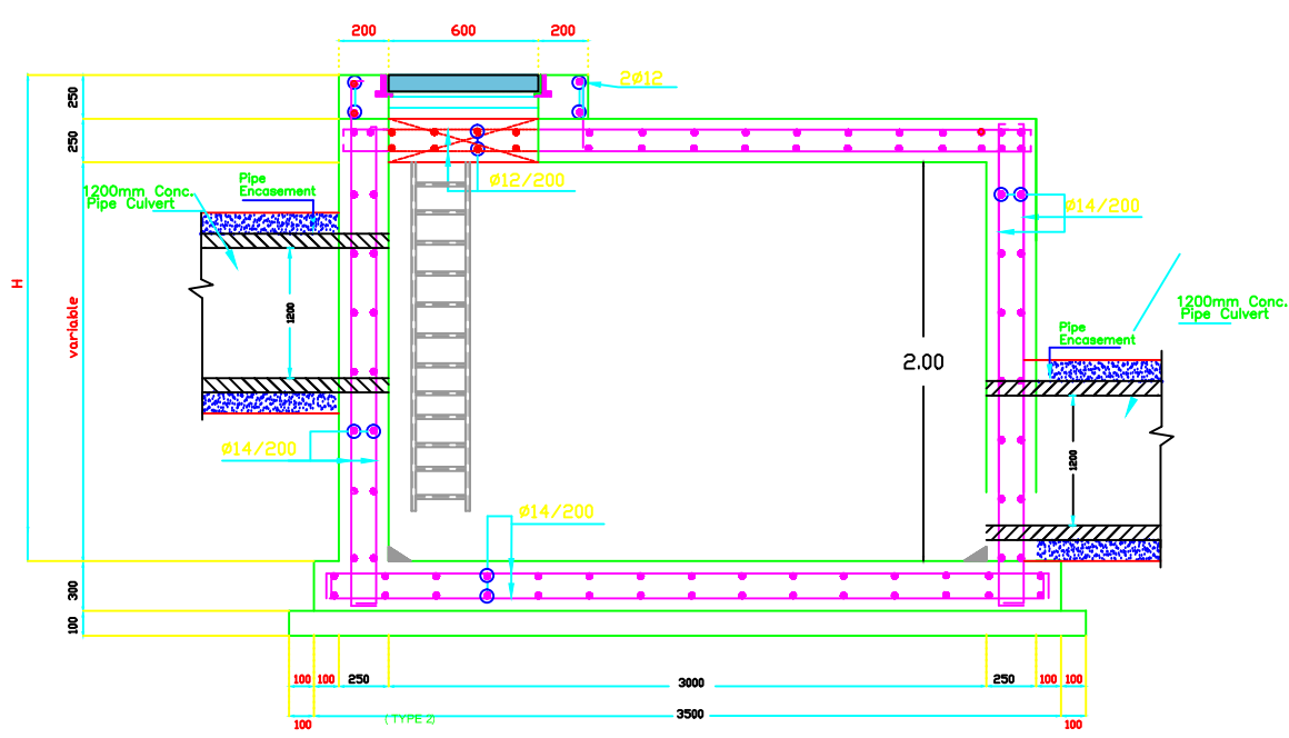
SECTION A-A SCALE 1/20 (FOR 1200 PIPE MANHOLES) (TYPE 2)
