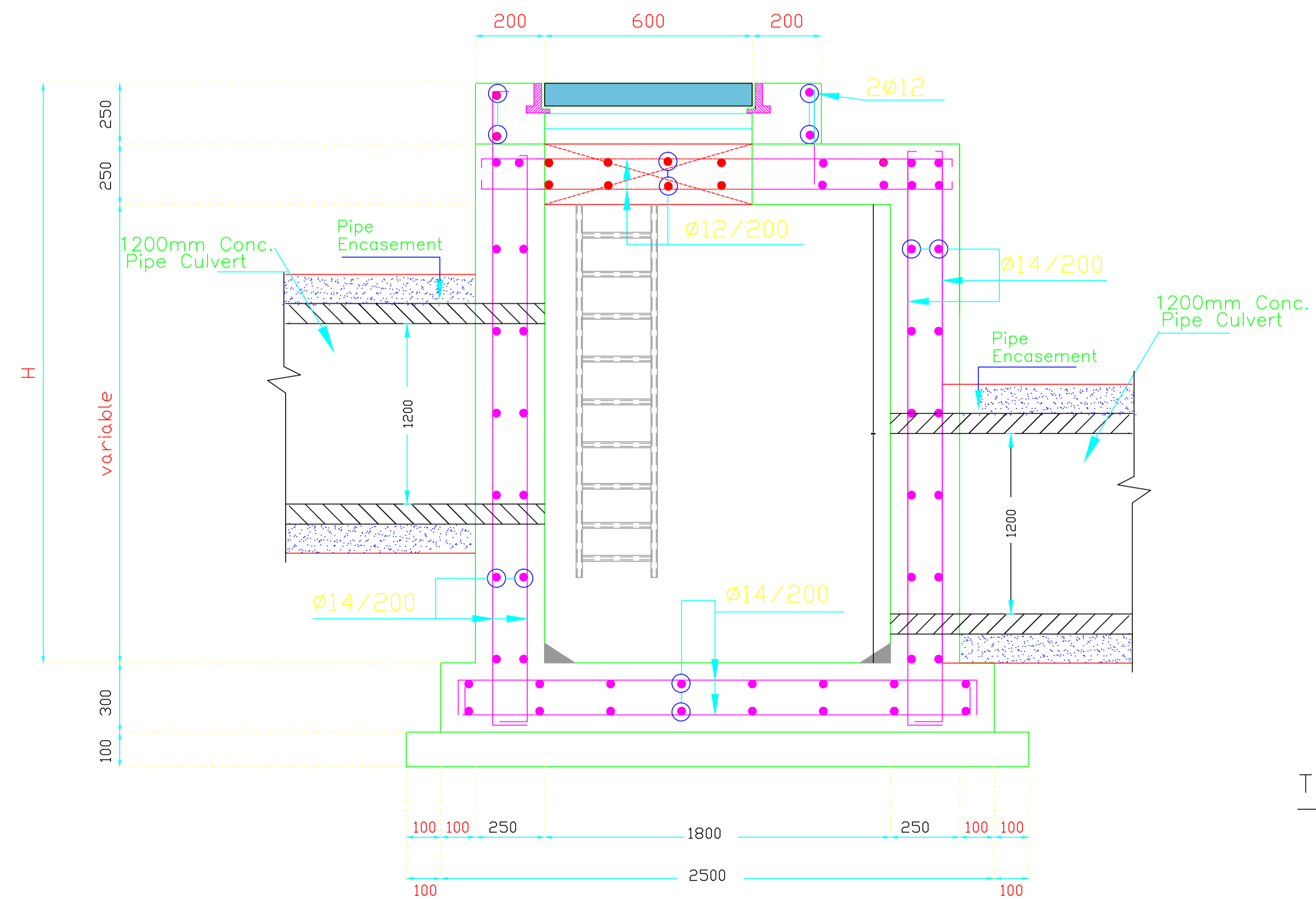
SECTION A-A SCALE 1/20 (FOR 1200 PIPE MANHOLES)
