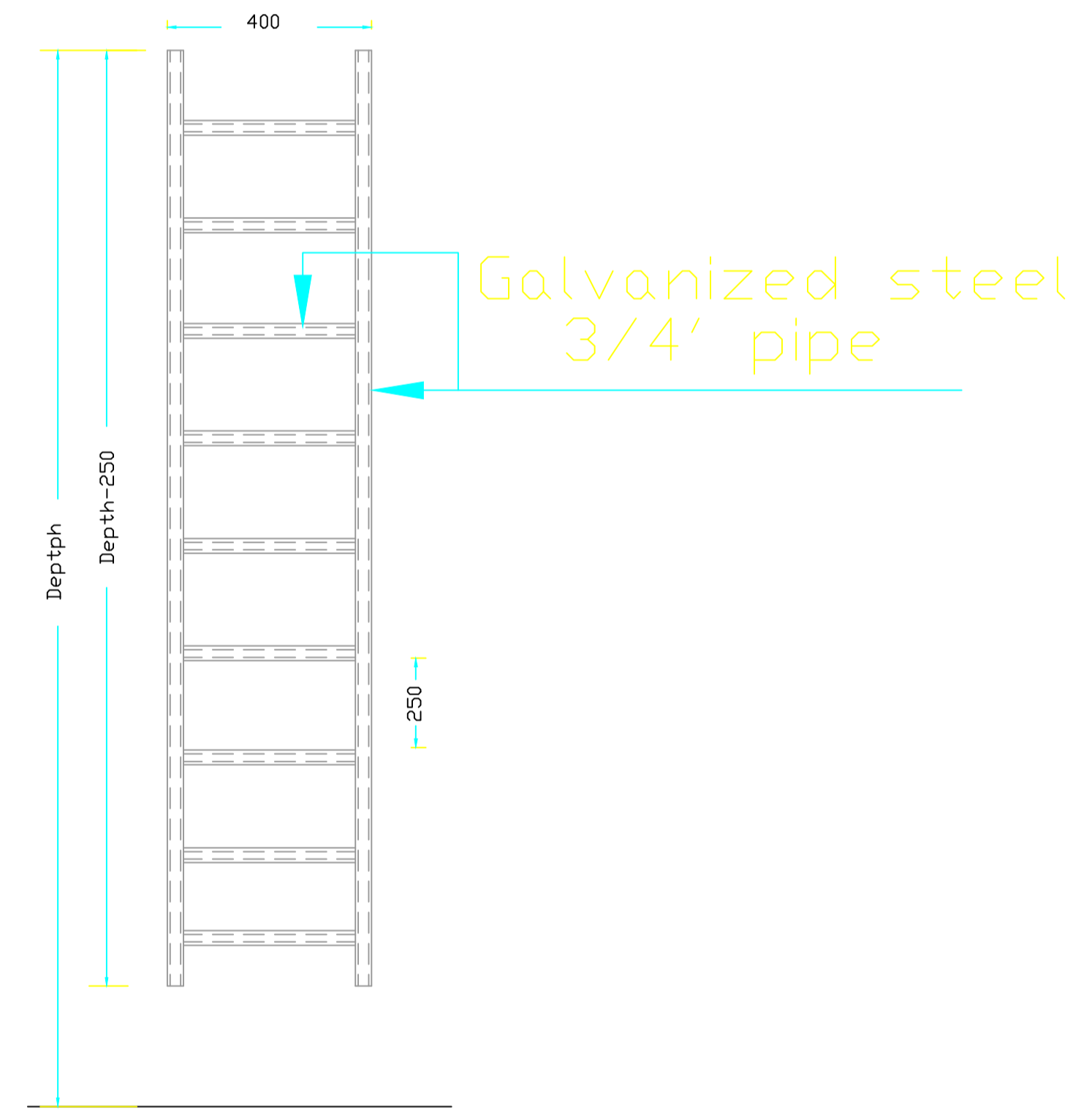
THE INSIDE STEEL STAIR DETAIL
