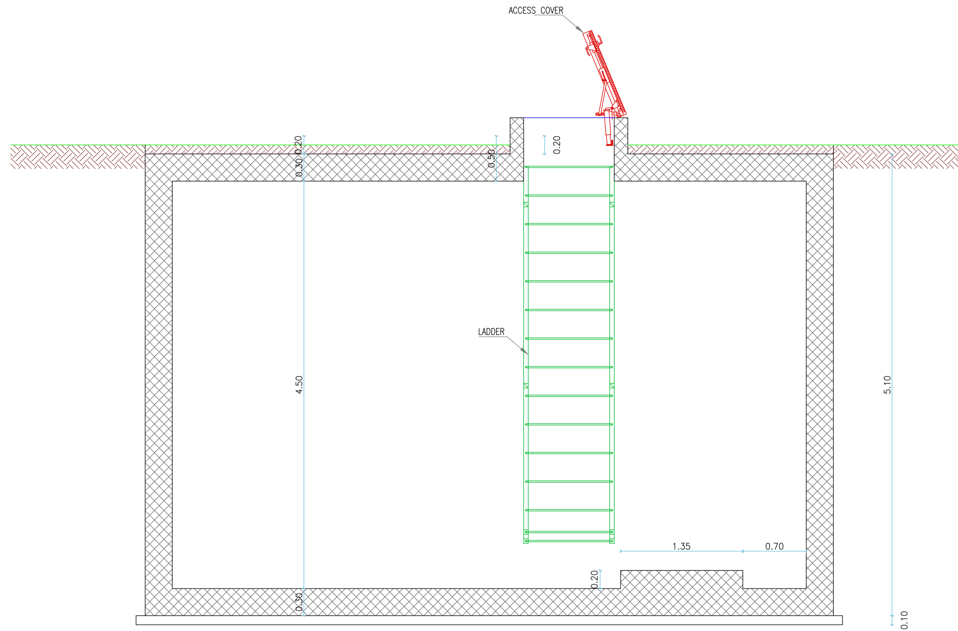
WATER TANK SECTION A-A
