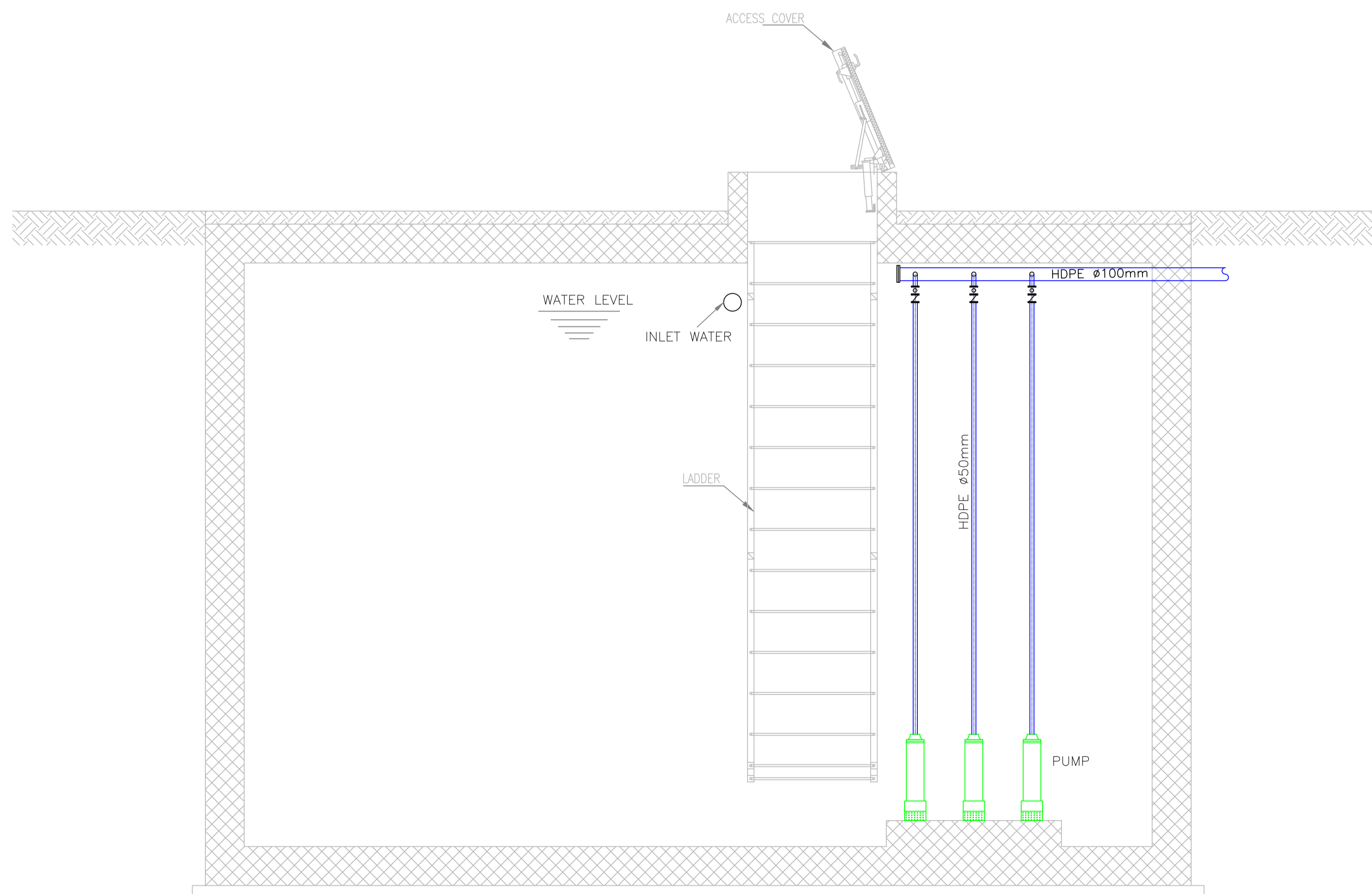
WATER TANK SECTION A-A
