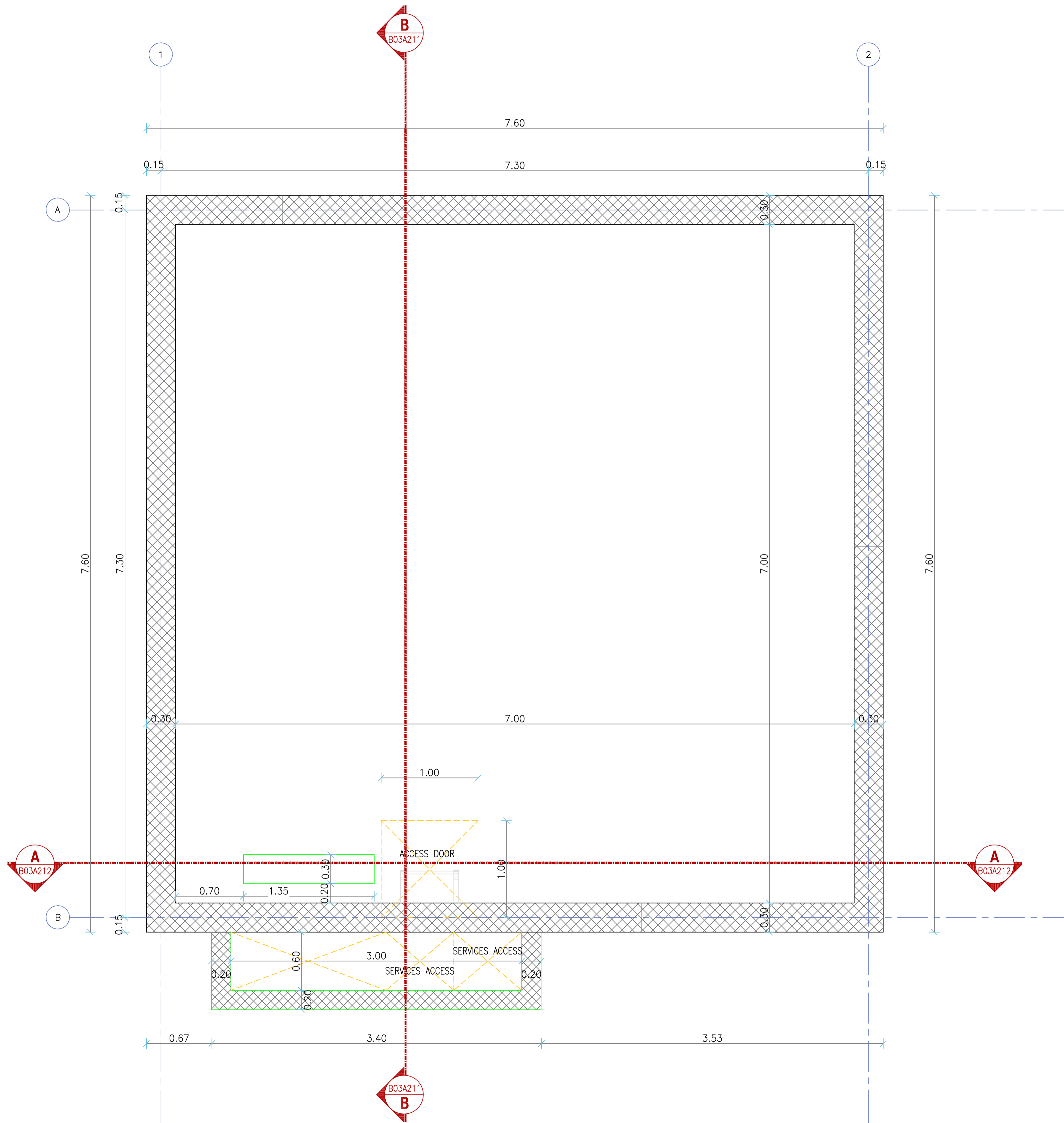
WATER TANK GEOMETRIC PLAN
