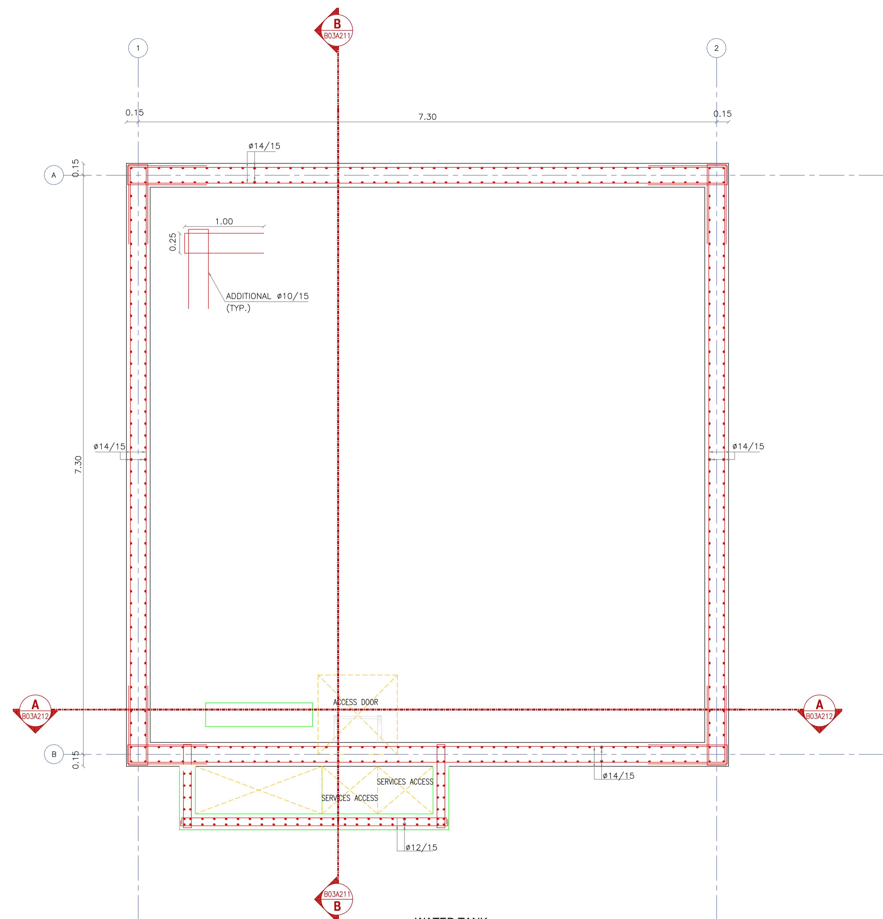
WATER TANK WALL REINFORCEMENT PLAN
