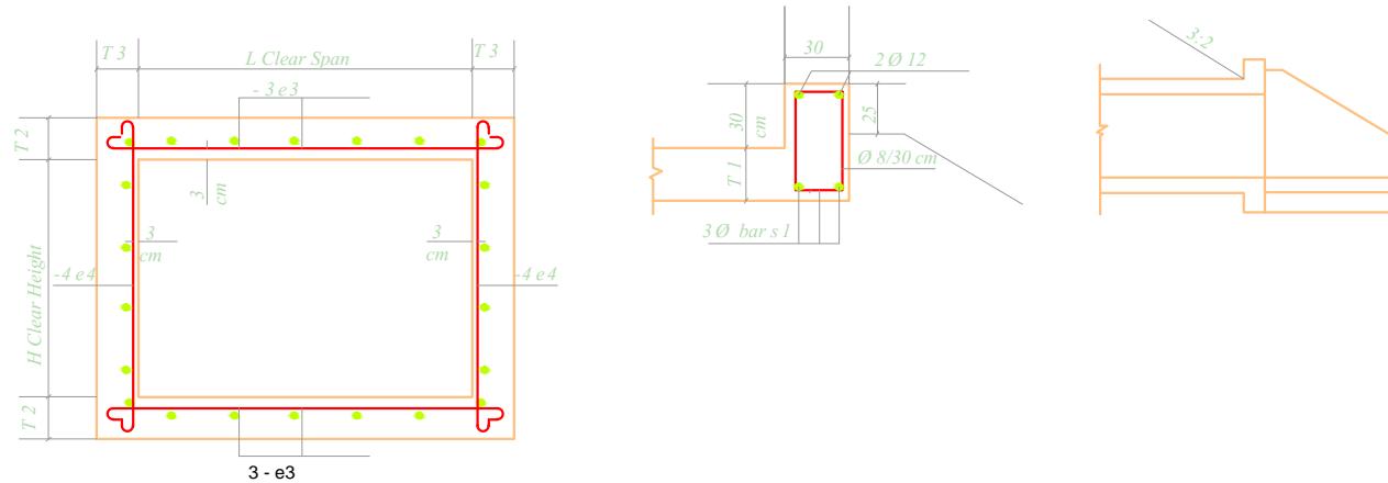
Typical Section
