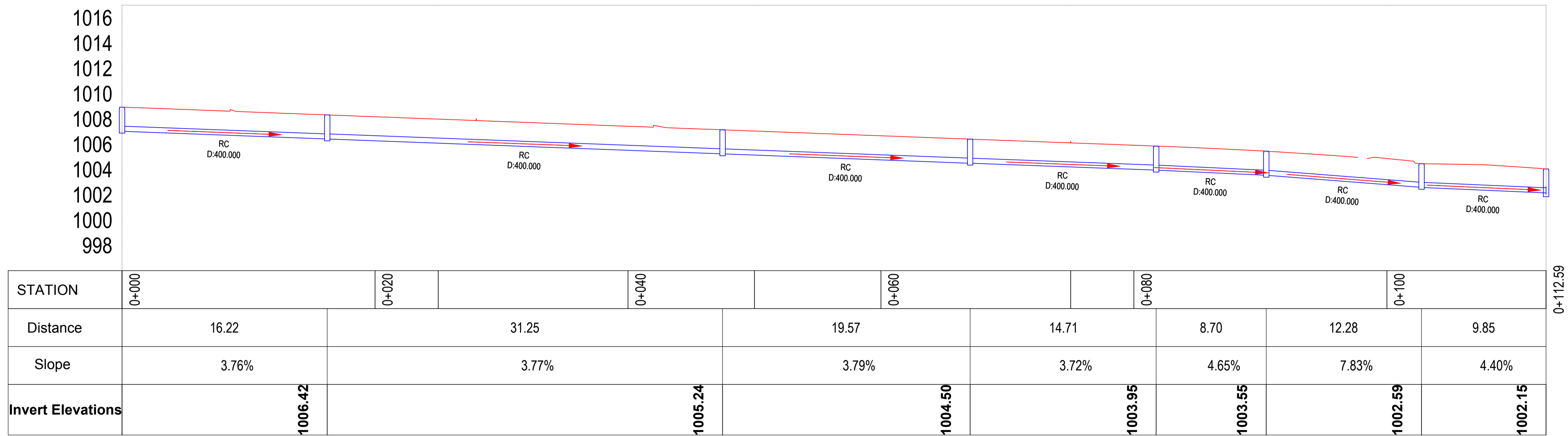
LINE PA-1 PROFILE
