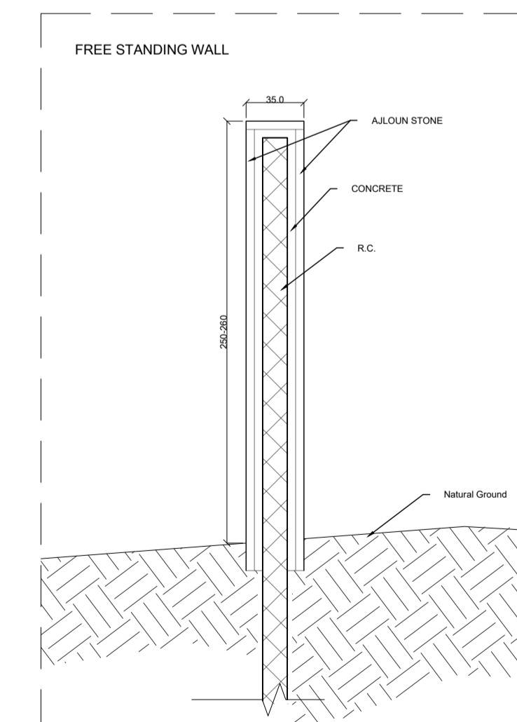
SECTION - S-21 SCALE:1-20
