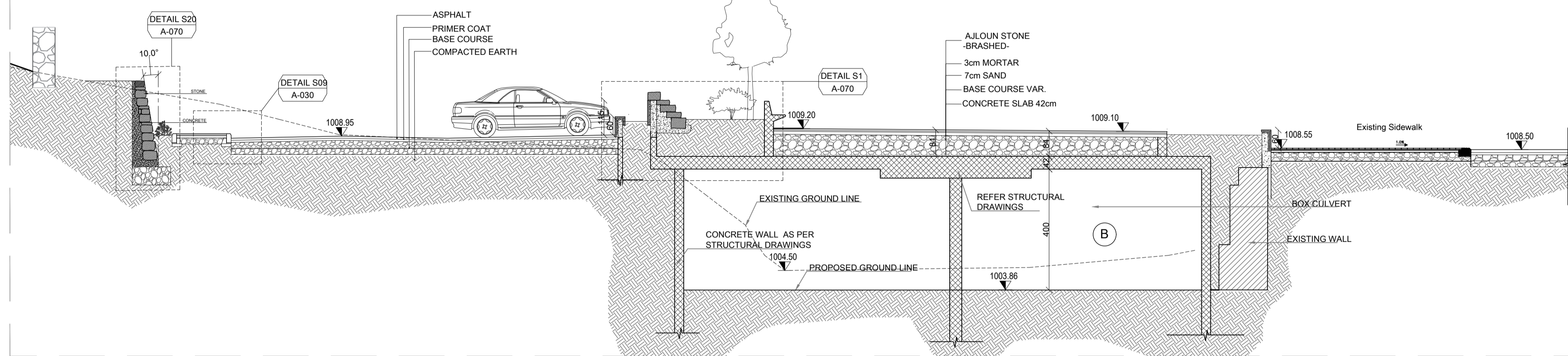
SECTION B-B
