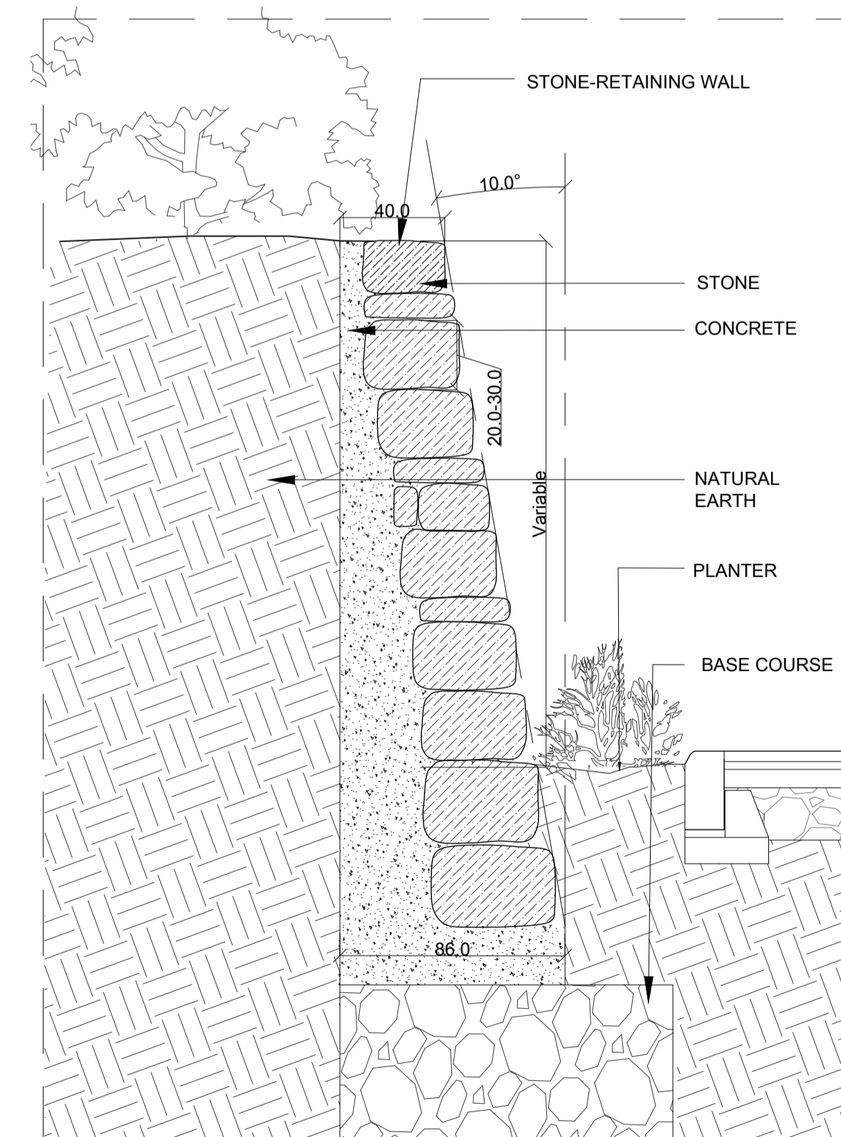
SECTION - S-20 SCALE:1-20
