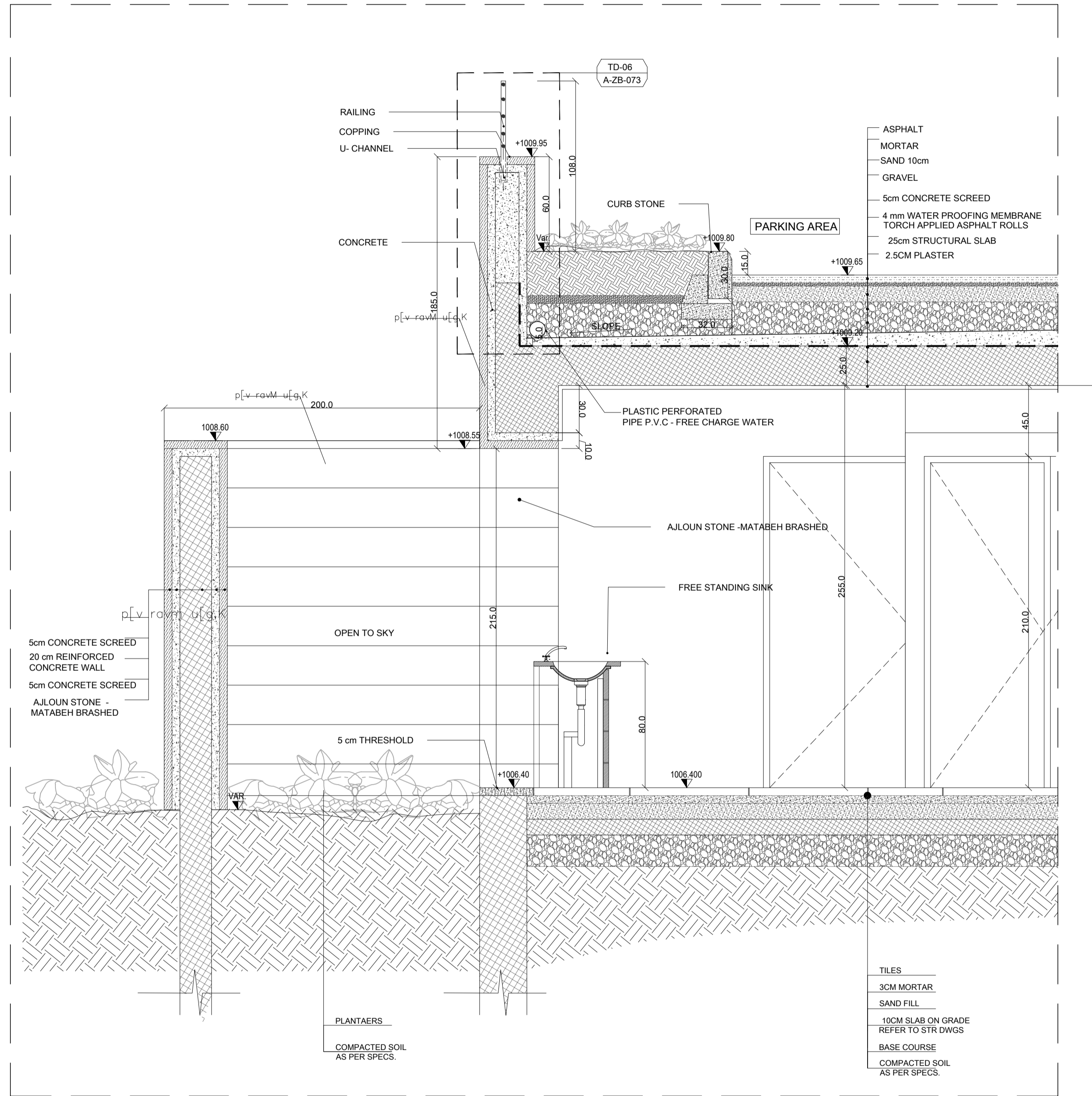
WALL SECTION 1 1:20
