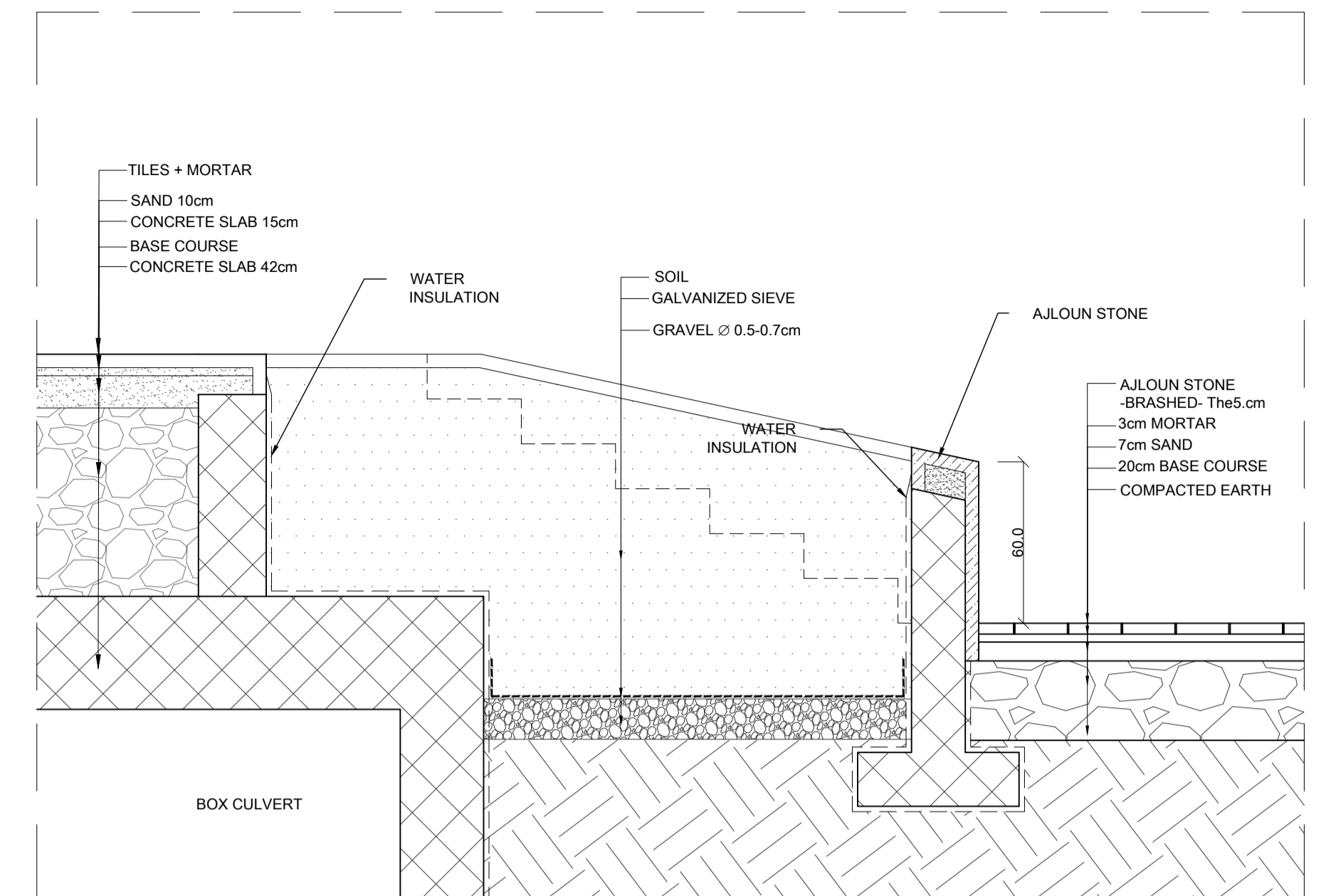
SECTION - S-14 SCALE:1-20
