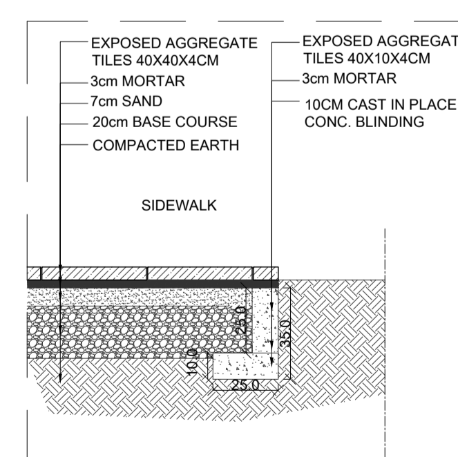
SECTION - S-19 SCALE:1-20
