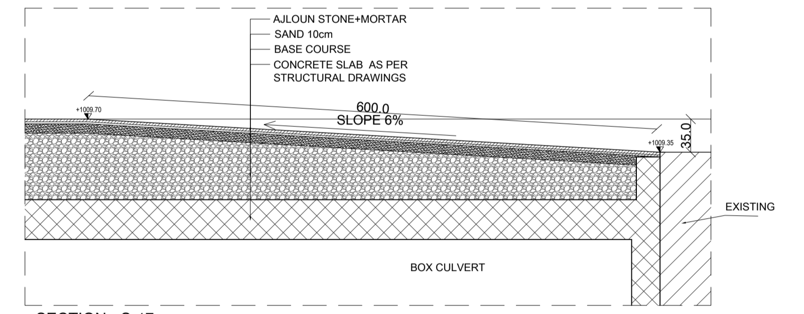
SECTION - S-17 SCALE:1-50
