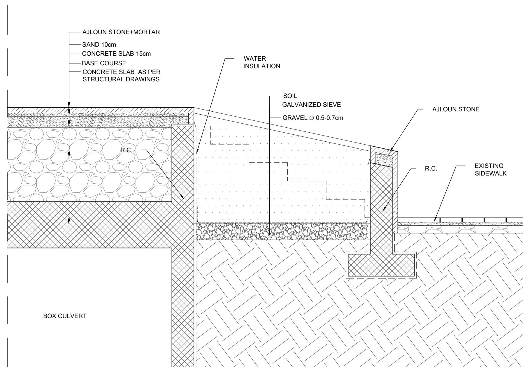
SECTION - S-12 SCALE:1-20
