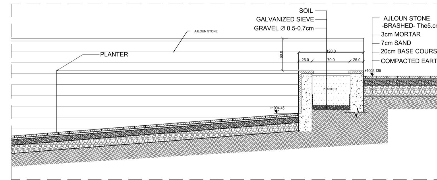
SECTION - S-16 SCALE:1-50
