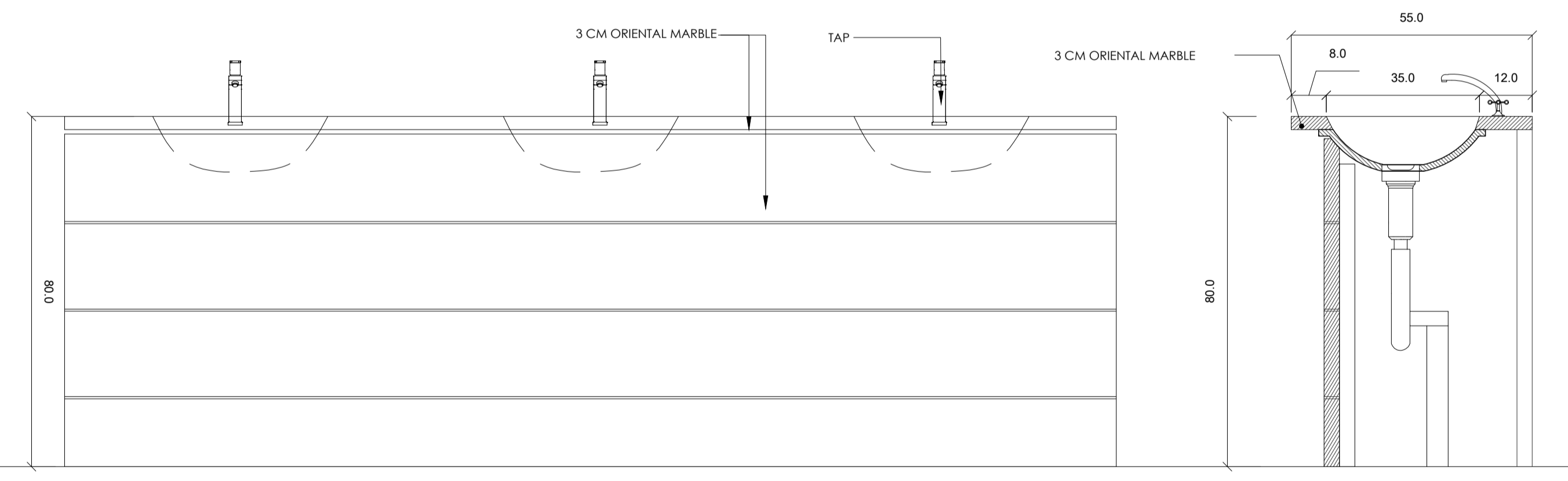
SINK DETAILS 1:10
