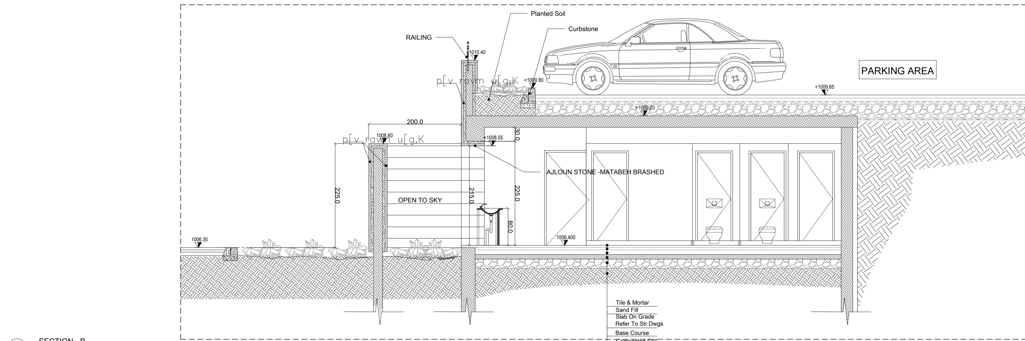
SECTION - B 1:50
