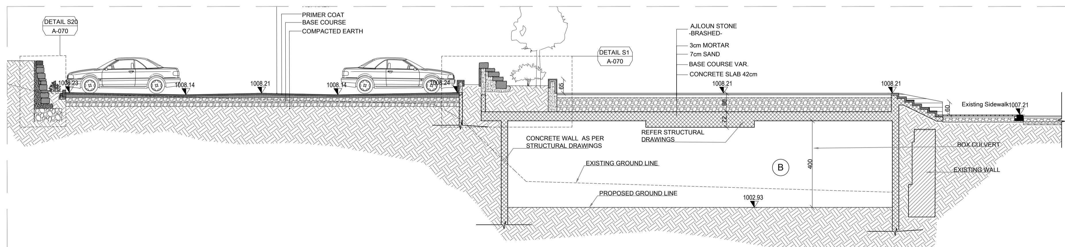
SECTION C-C
