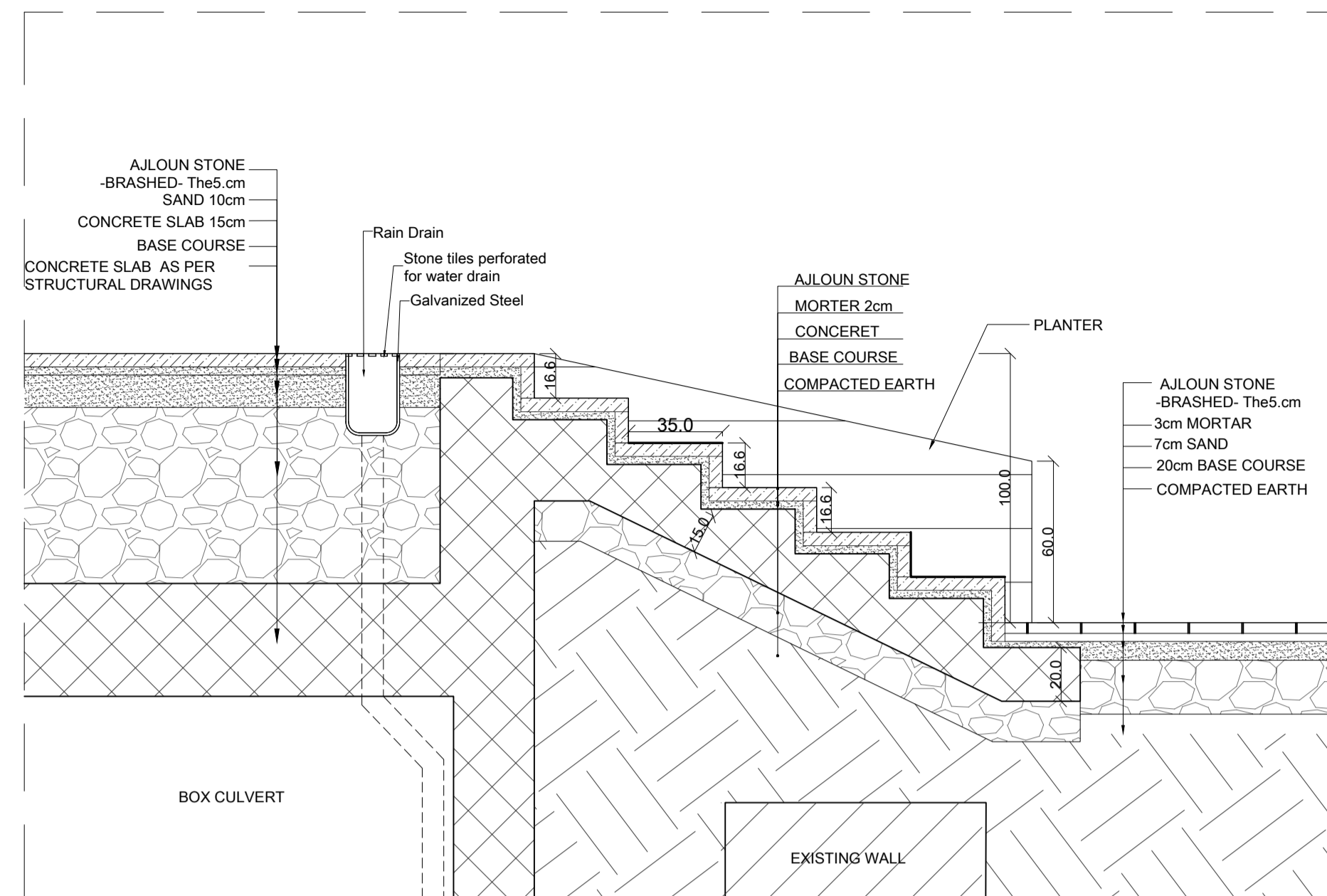
SECTION - S-13 SCALE:1-20
