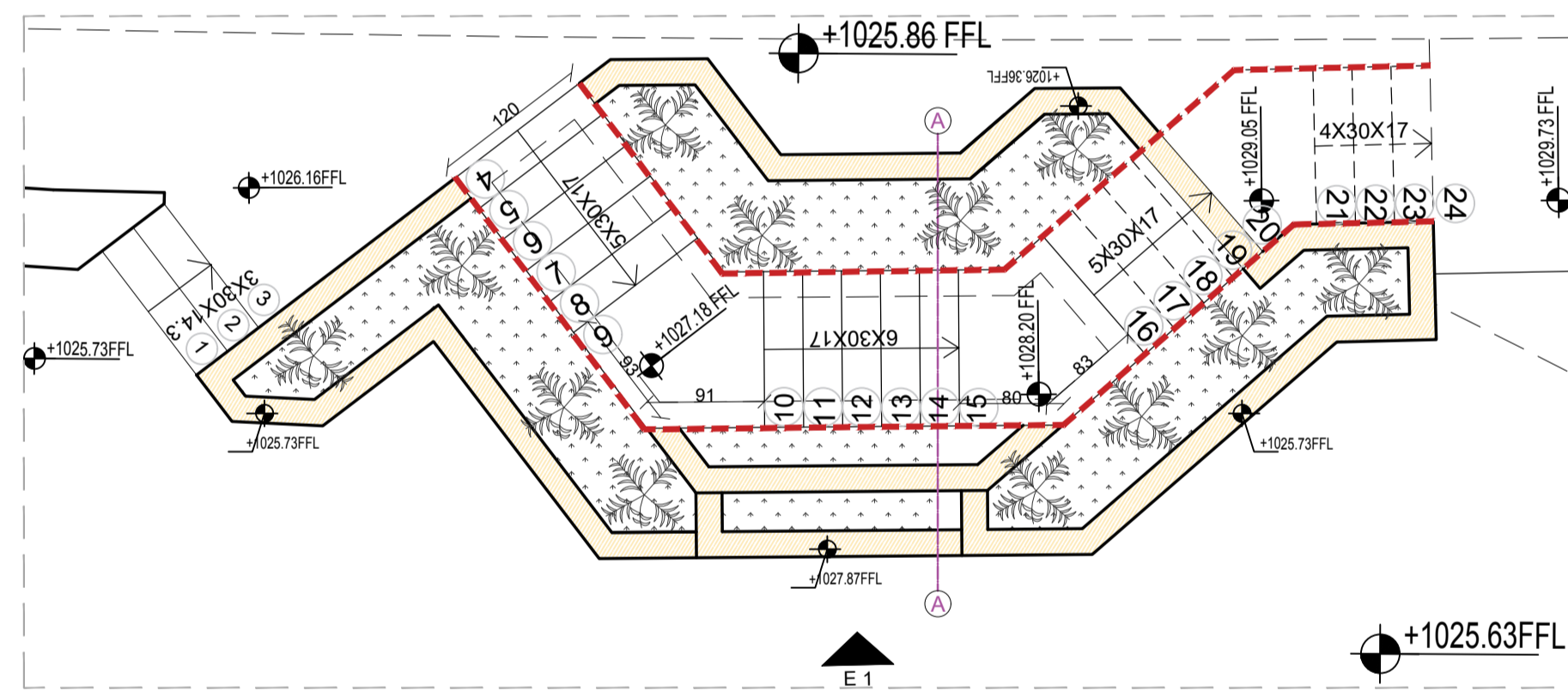
STAIRS 06-TOP VIEW SCALE:1-50
