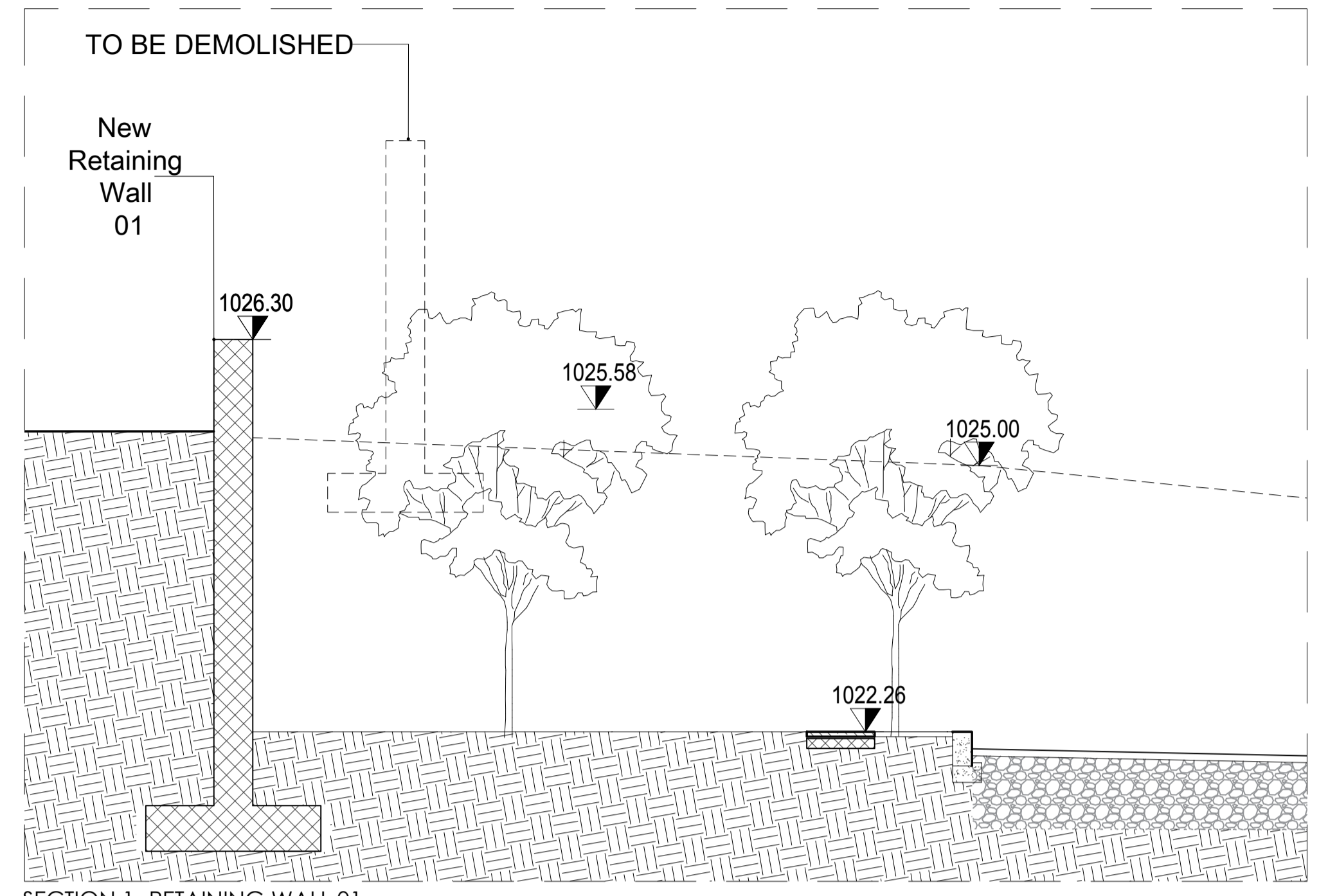
SECTION 1 - RETAINING WALL 01 SCALE:1-50
