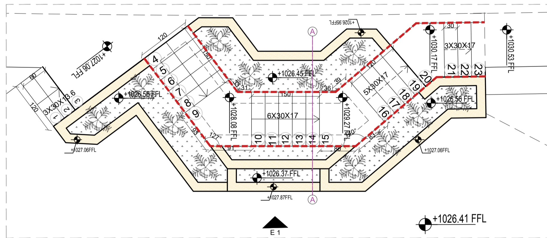
STAIRS 05-TOP VIEW SCALE:1-50
