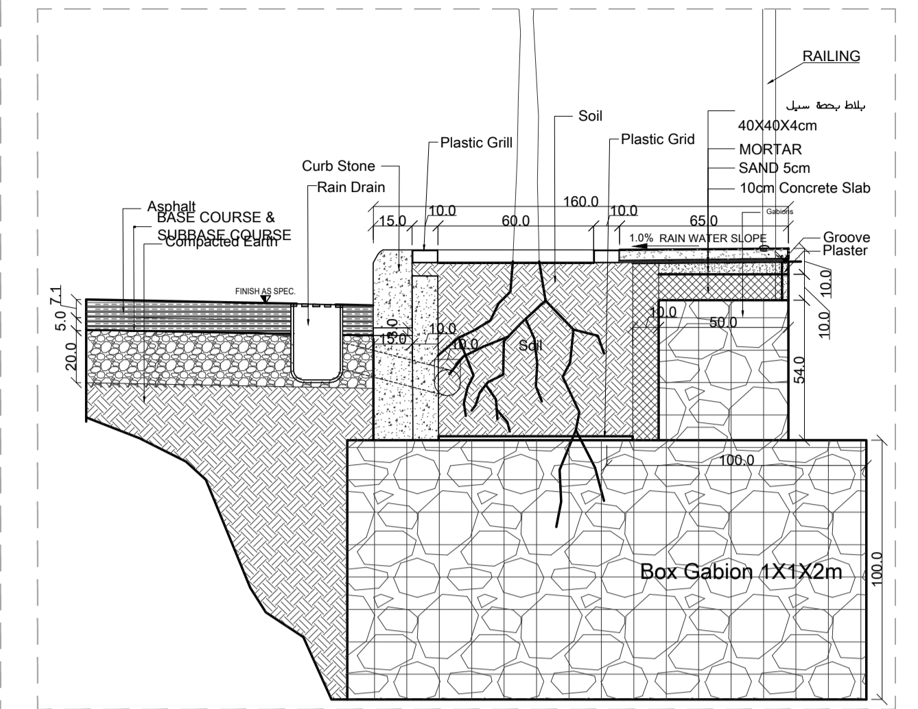
DETAIL 02 SCALE:1-20
