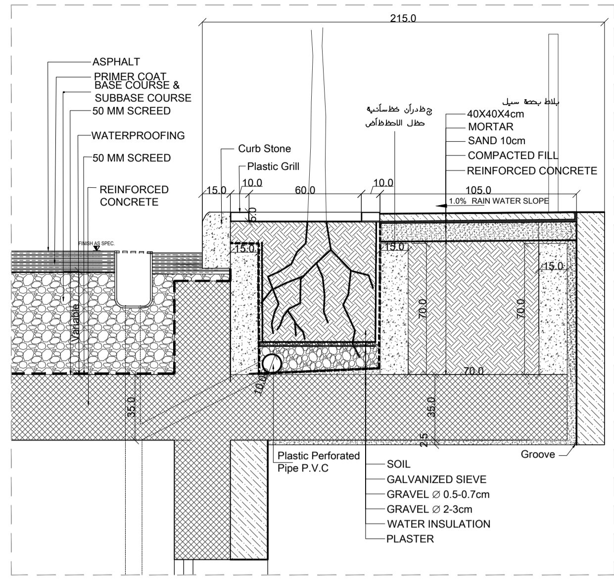
DETAIL 01 SCALE:1-20
