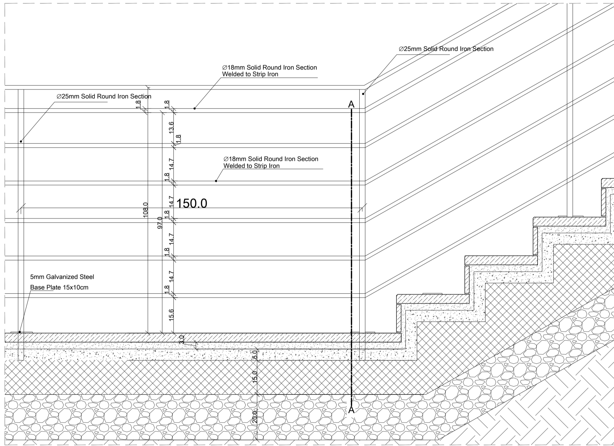
DETAIL 10 RAILING STAIRS DETAIL SCALE:1-10
