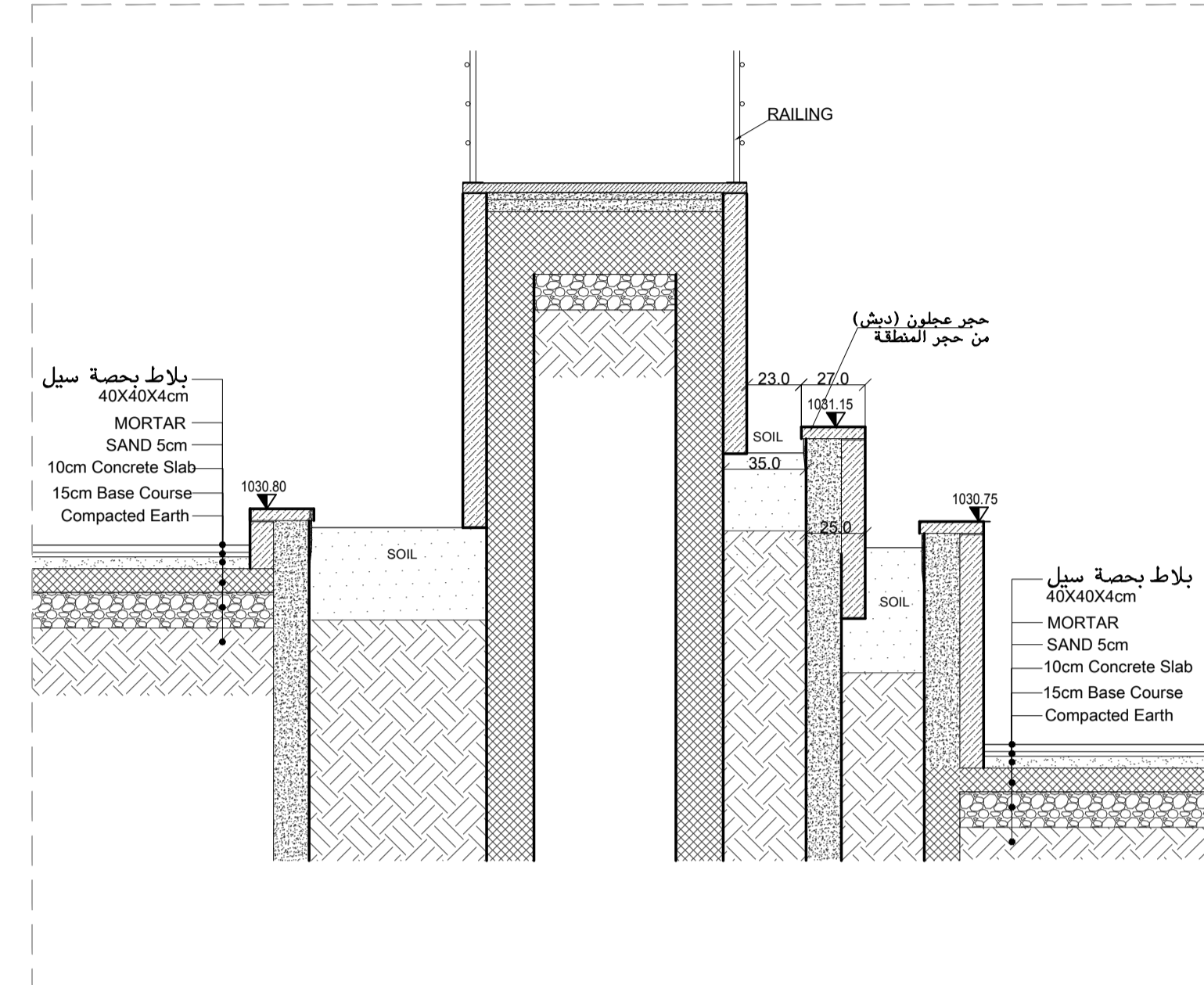
STAIRS 04-SECTION A-A SCALE:1-25
