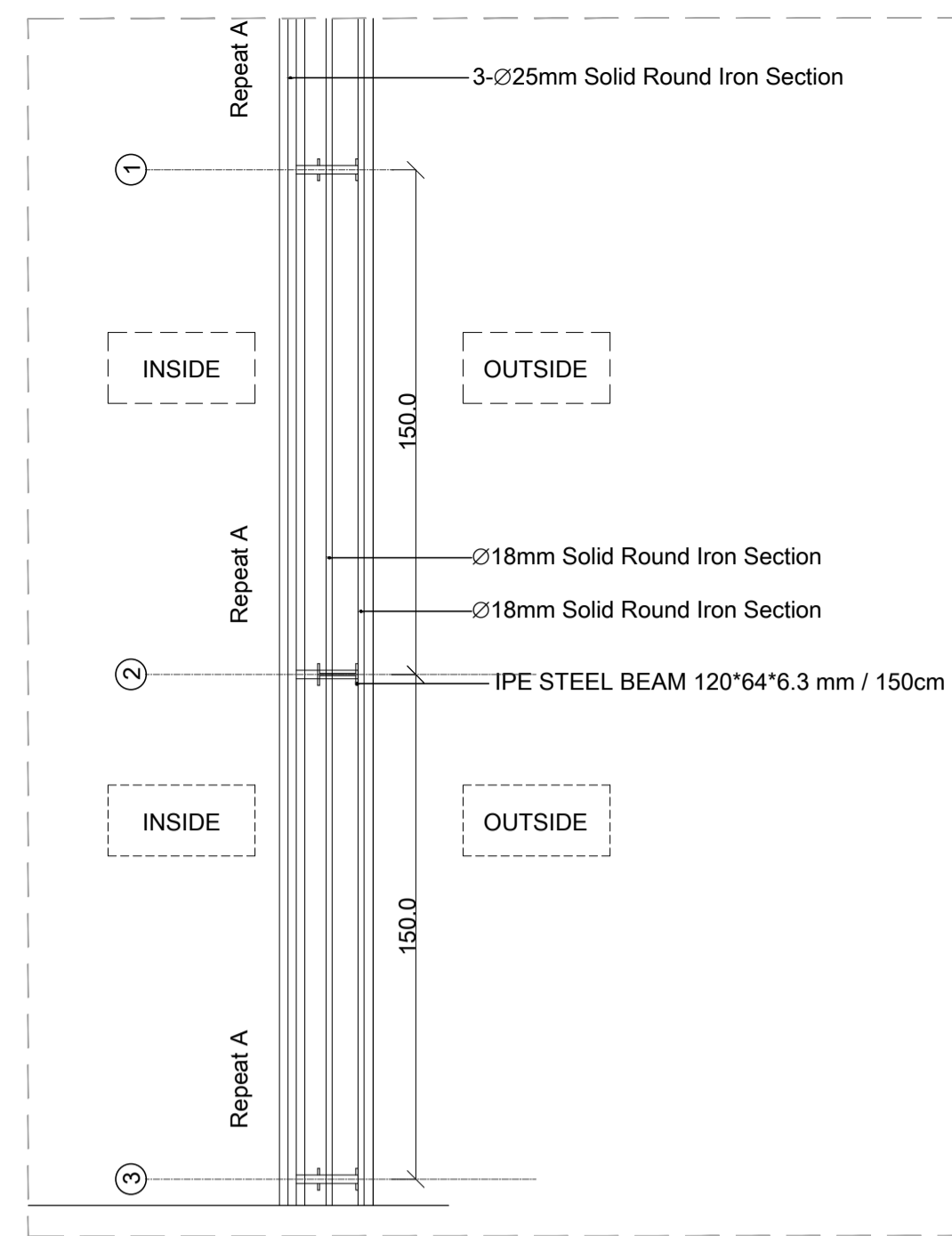
DETAIL 09 RAILING EDGE DETAIL - PLAN SCALE:1-20
