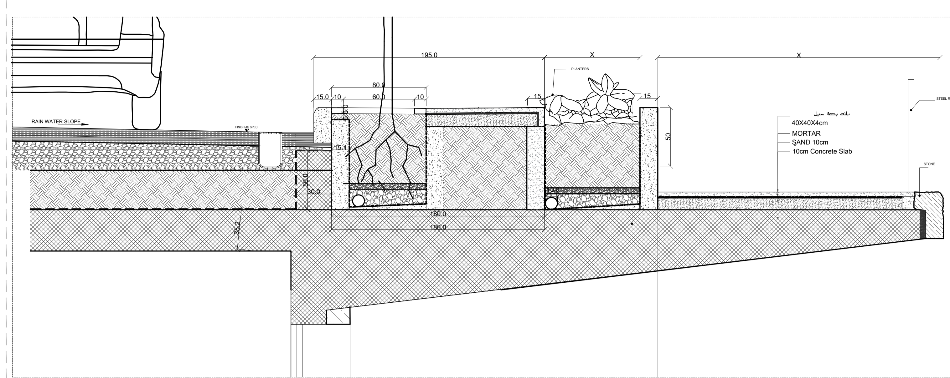
DETAIL 02 SCALE:1-20
