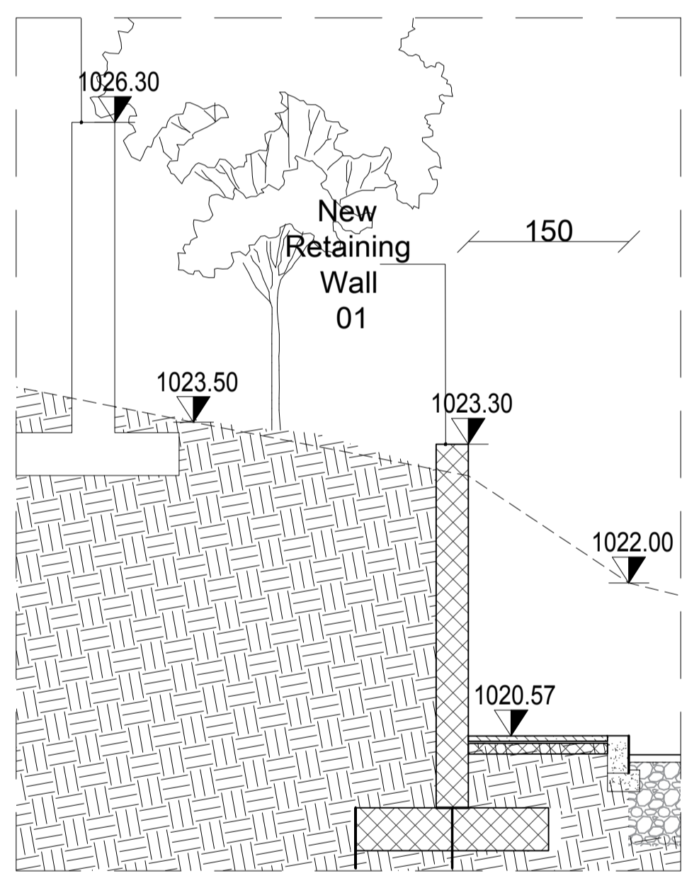
SECTION 2 - RETAINING WALL 01 SCALE:1-50
