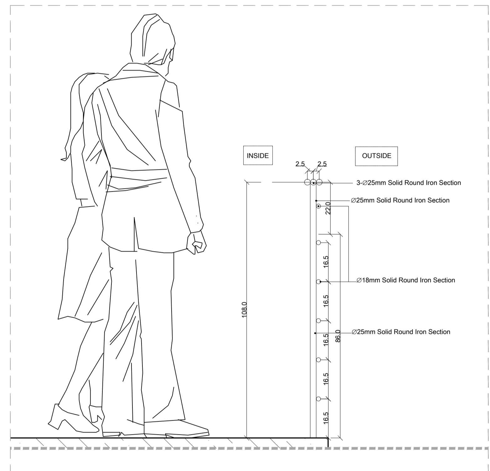
DETAIL 10 RAILING STAIRS DETAIL - SECTION - A SCALE:1-10
