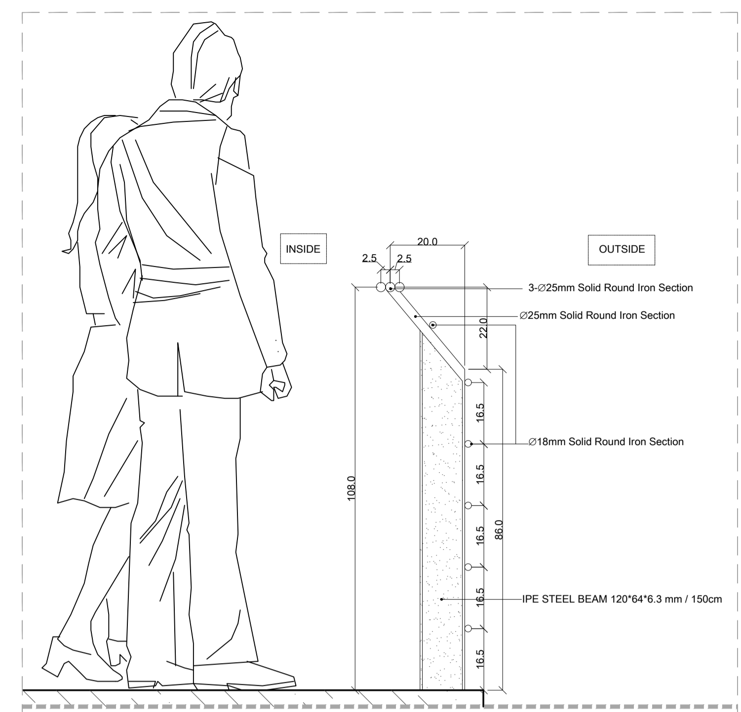
DETAIL 09 RAILING EDGE DETAIL - SECTION SCALE:1-10
