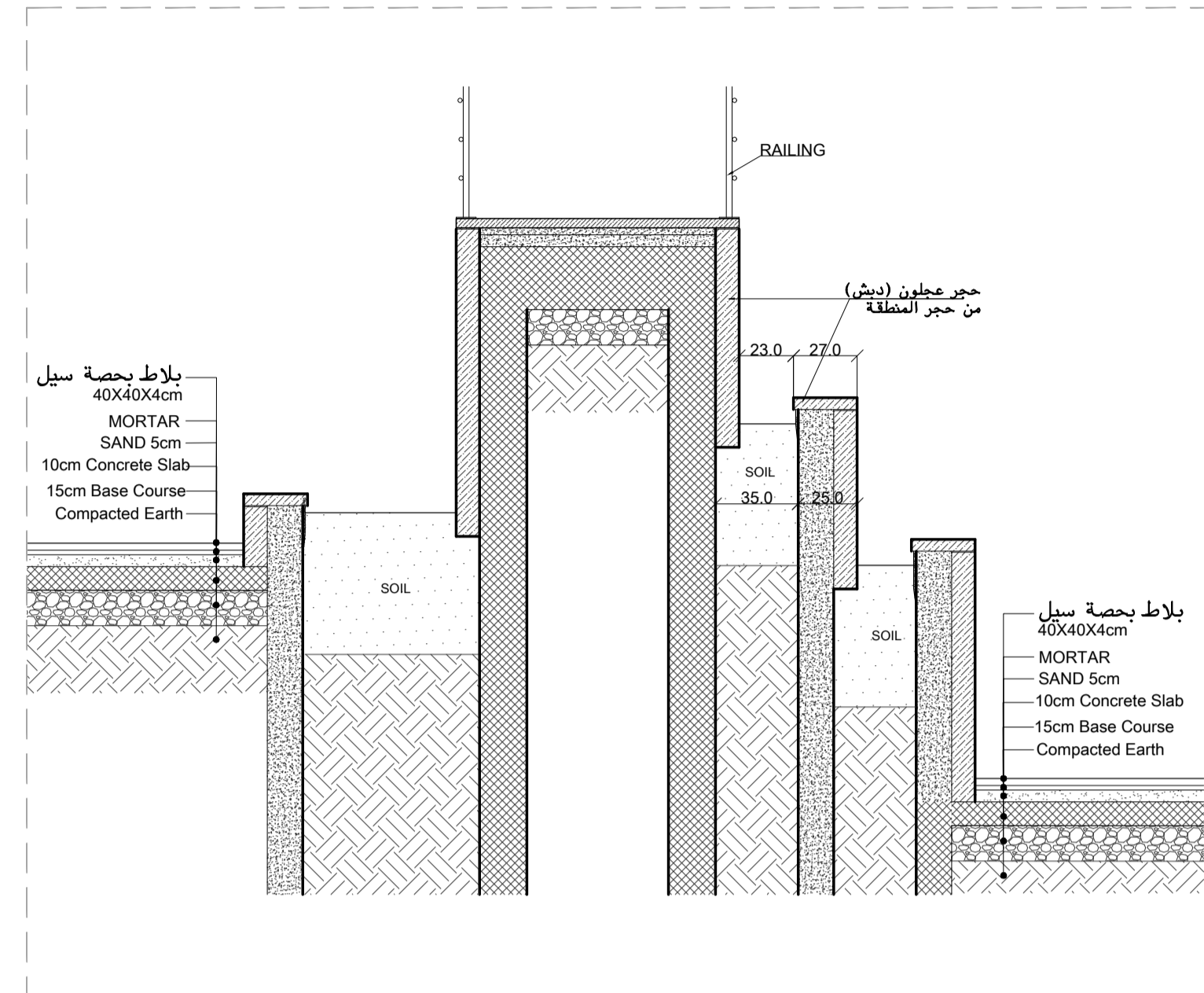
STAIRS 05-SECTION A-A SCALE:1-25
