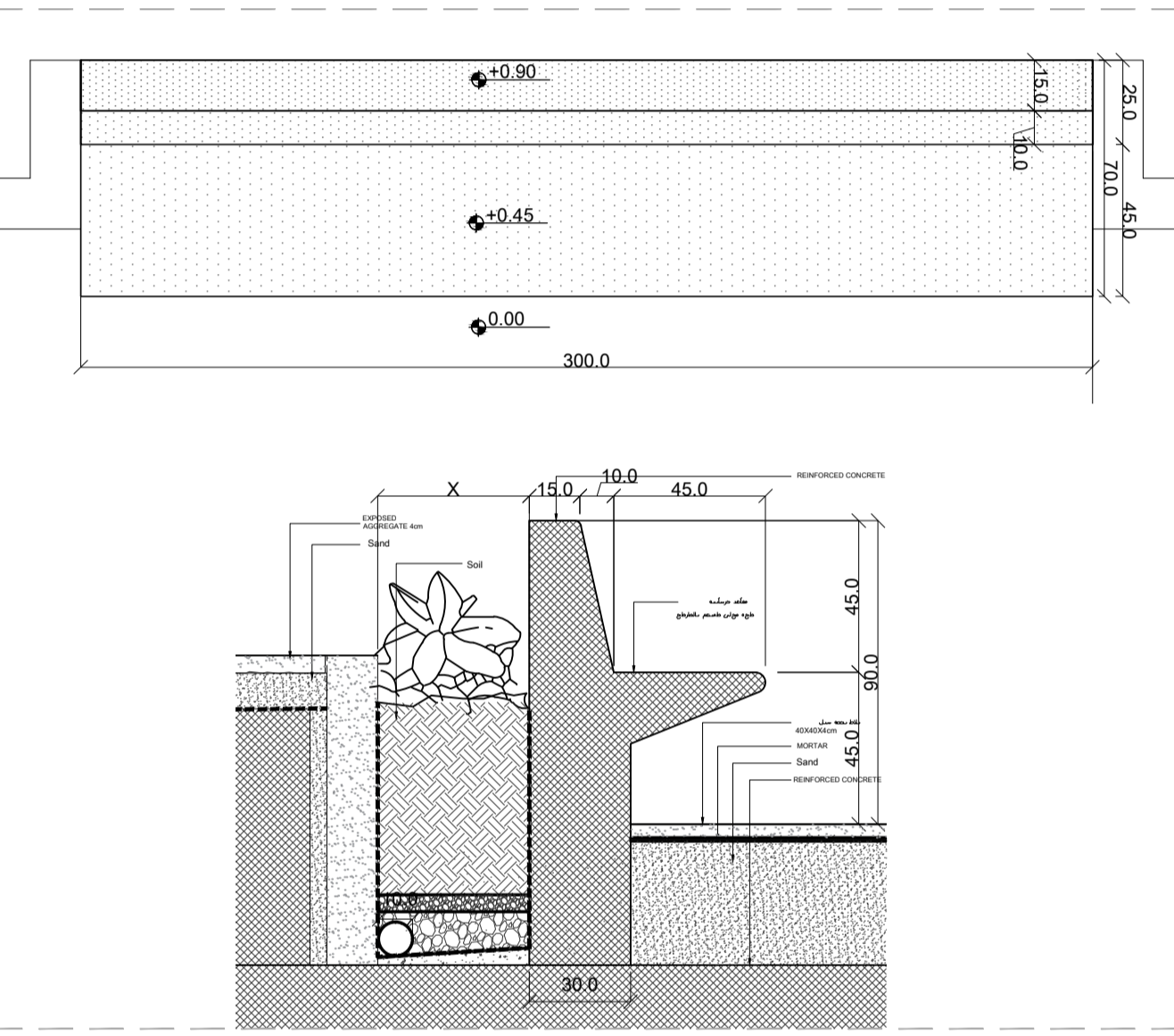
DETAIL 03 SCALE:1-20
