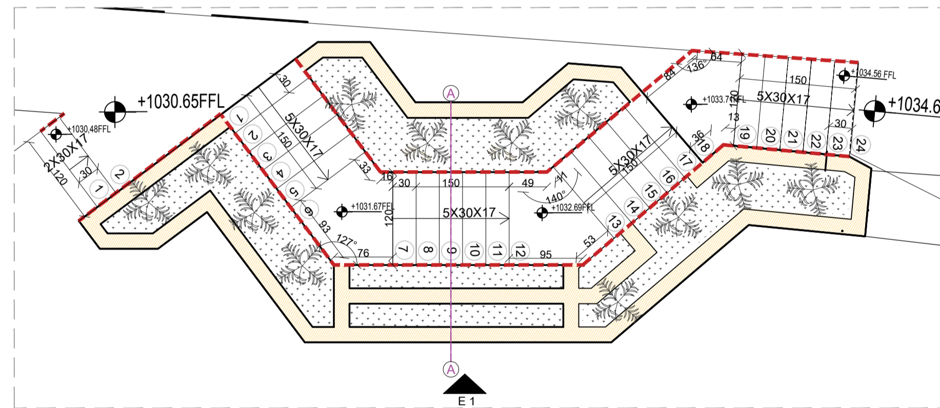
STAIRS 04-TOP VIEW SCALE:1-50
