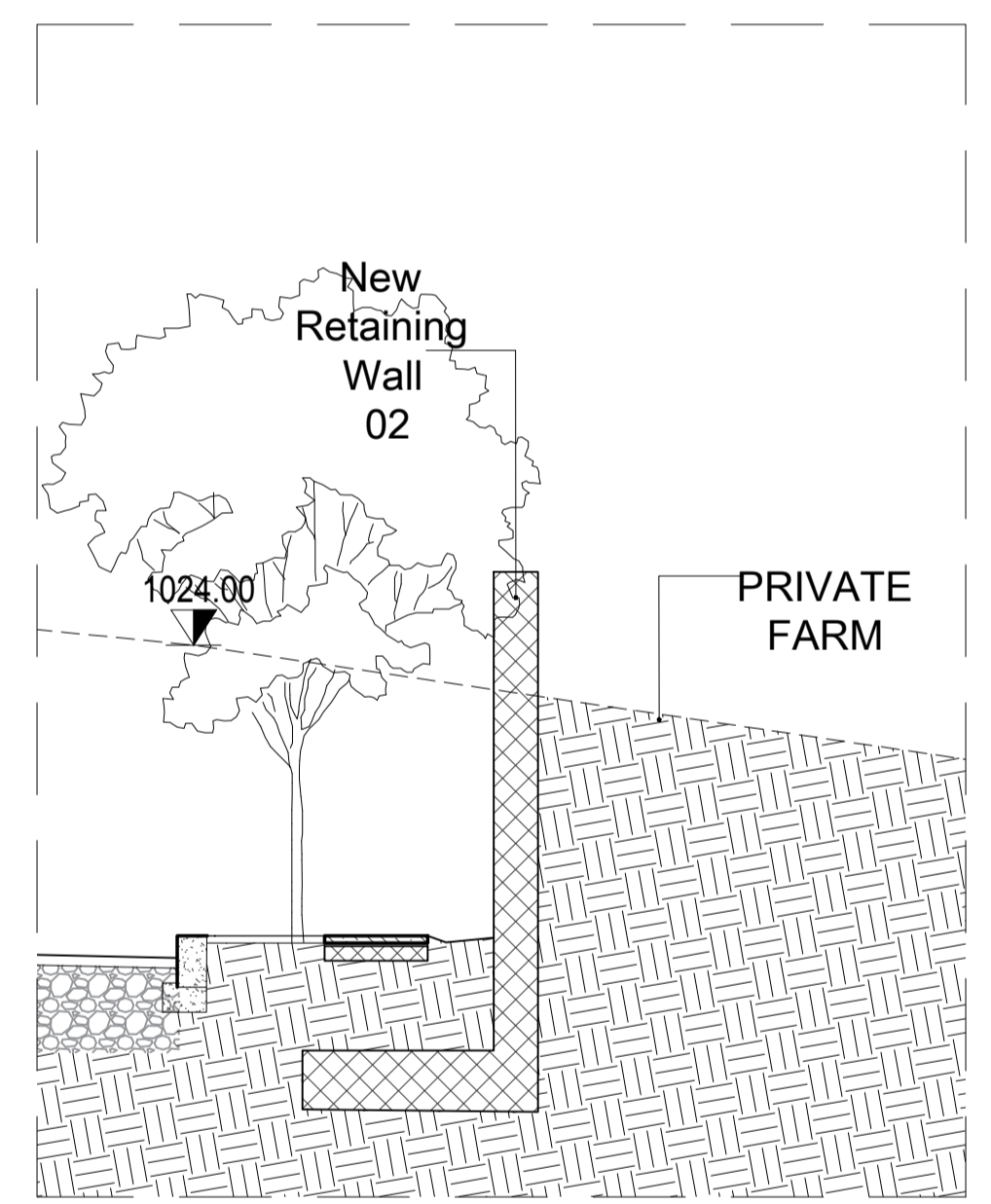
SECTION 1 - RETAINING WALL 02 SCALE:1-50
