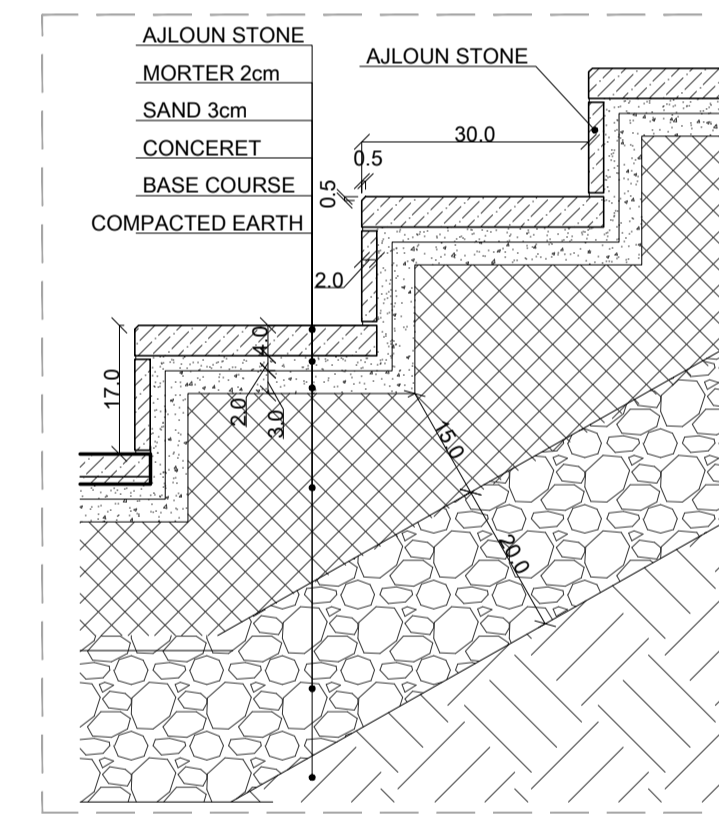
STAIRS 05-DETAIL 01 SCALE:1-10
