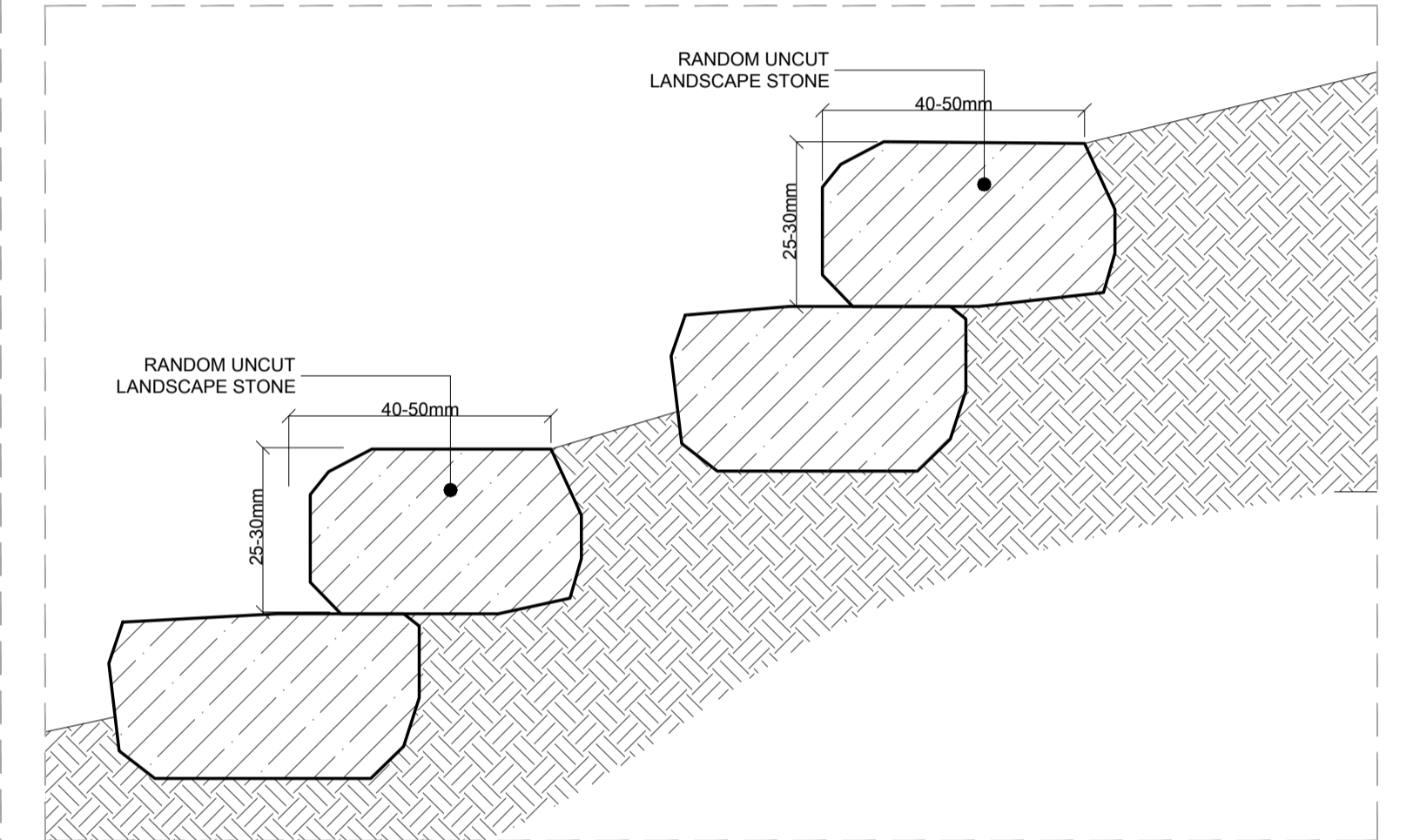
DETAIL 06 SCALE:1-10
