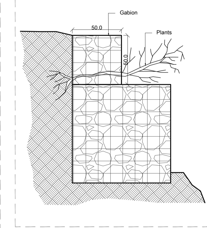
DETAIL 07 SCALE:1-20
