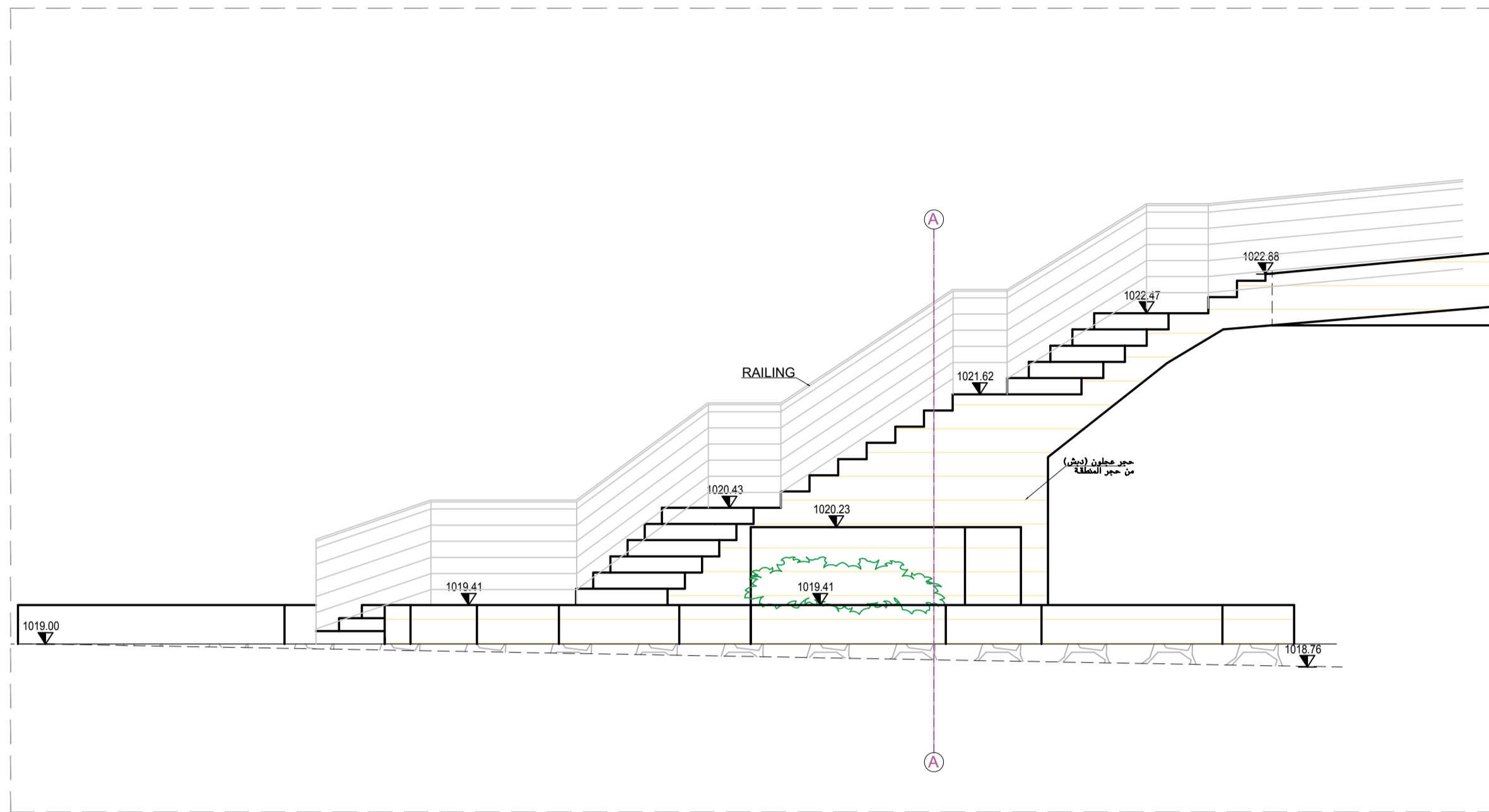
STAIRS 05-ELEVATION 1 SCALE:1-50
