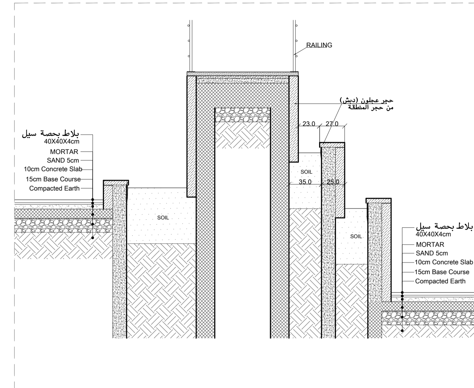
STAIRS 06-SECTION A-A SCALE:1-25
