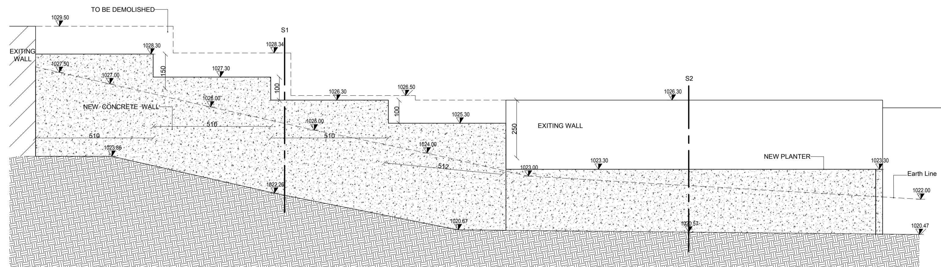
ELEVATION - RETAINING WALL 01 SCALE:1-100
