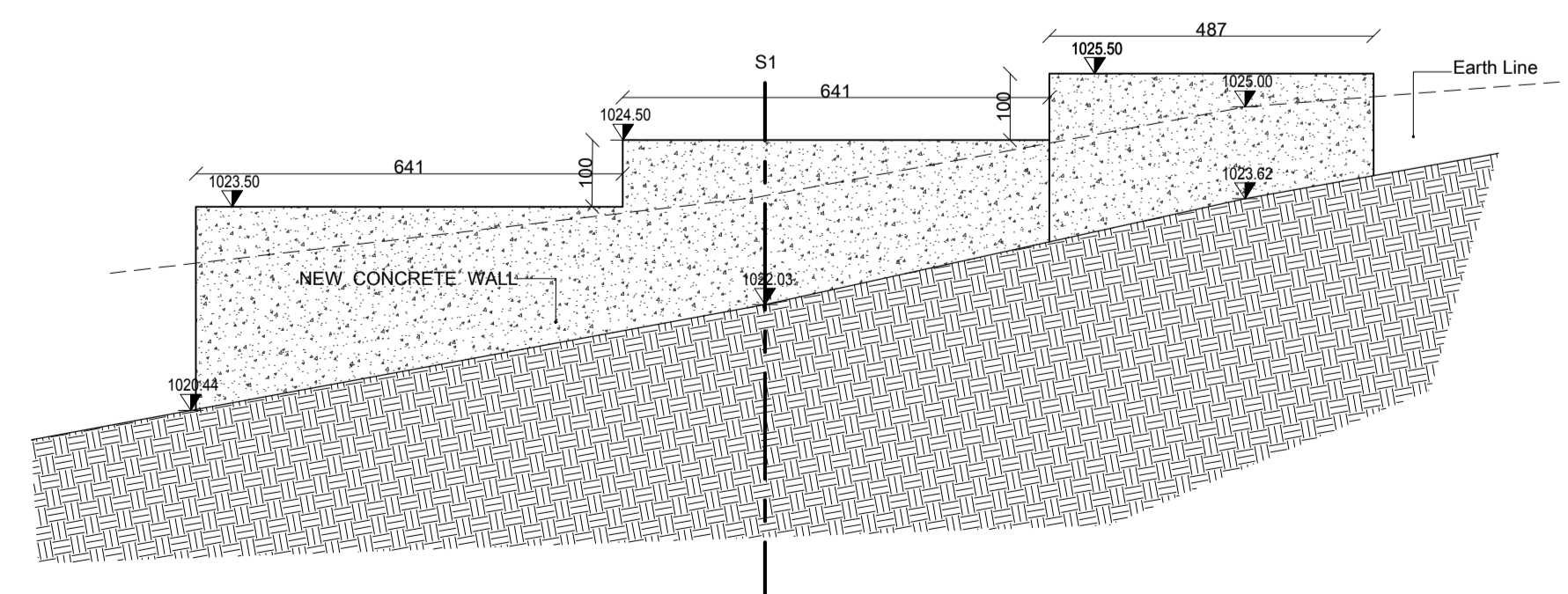
ELEVATION - RETAINING WALL 02 SCALE:1-100
