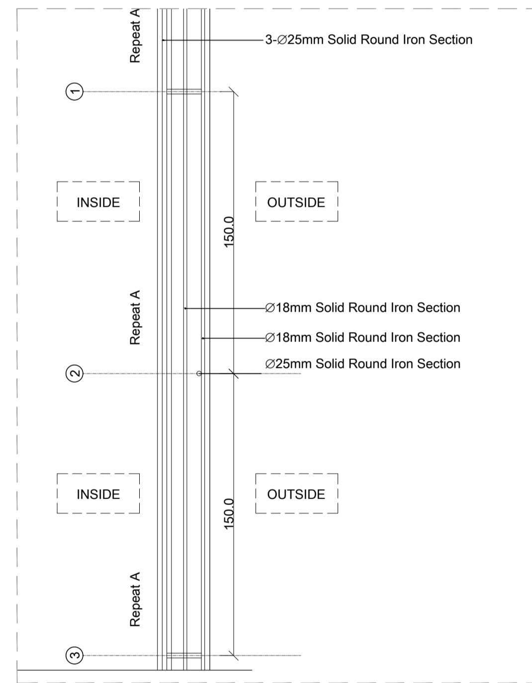
DETAIL 10 RAILING STAIRS DETAIL - PLAN SCALE:1-20
