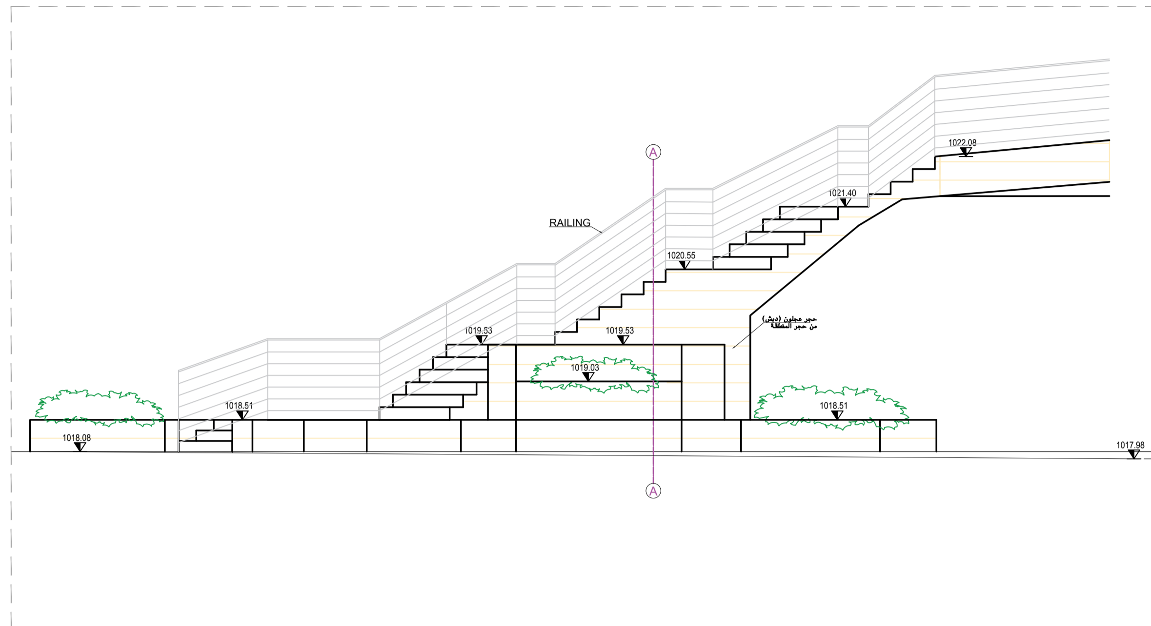
STAIRS 06-ELEVATION 1 SCALE:1-50
