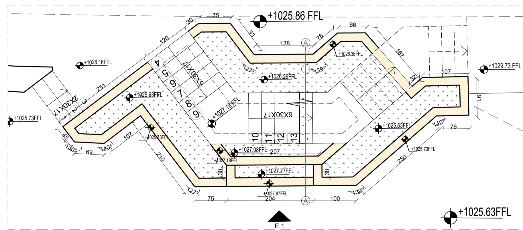
STAIRS 06-PLAN VIEW SCALE:1-50
