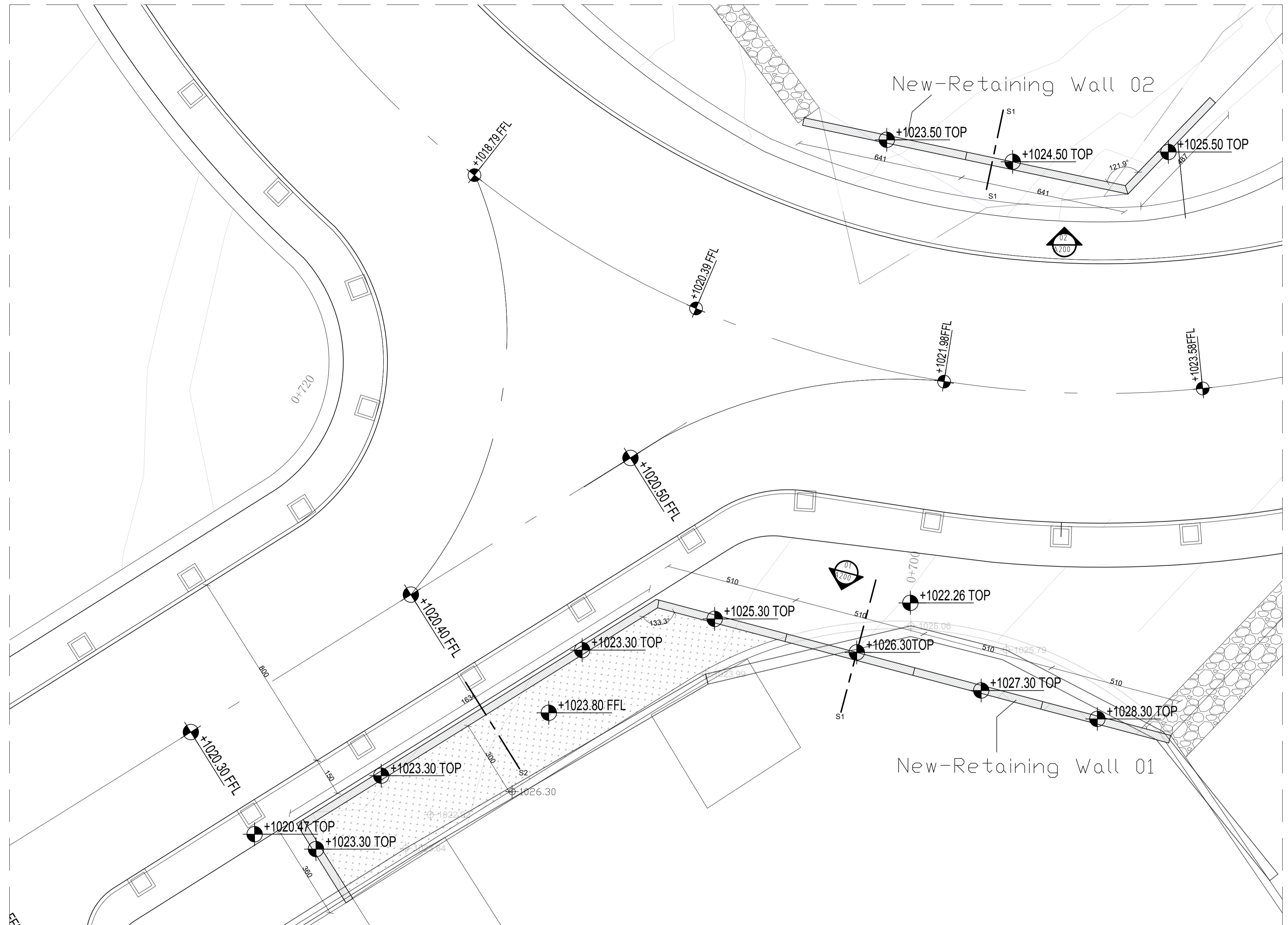
TOP VIEW SCALE:1-100
