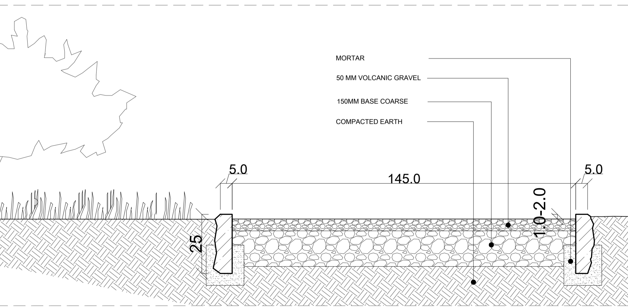
DETAIL 05 SCALE:1-10
