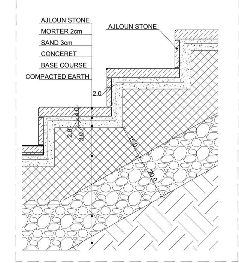
DETAIL 08 SCALE:1-10
