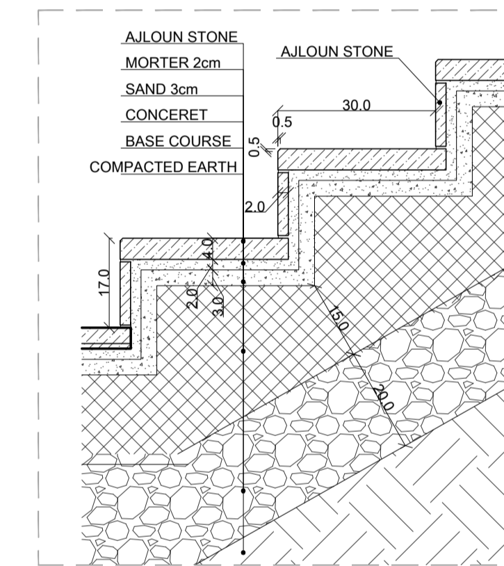
STAIRS 04-DETAIL 01 SCALE:1-10
