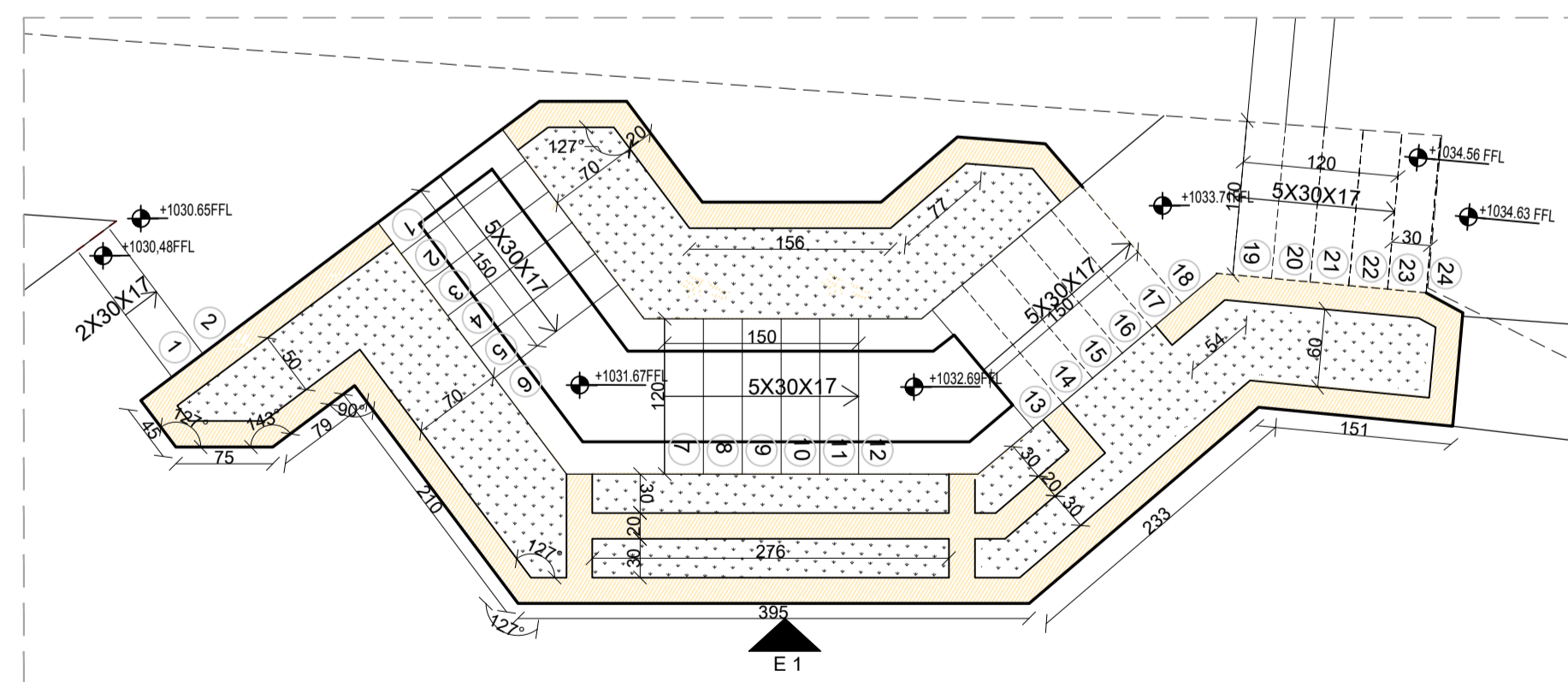
STAIRS 04-PLAN VIEW SCALE:1-50
