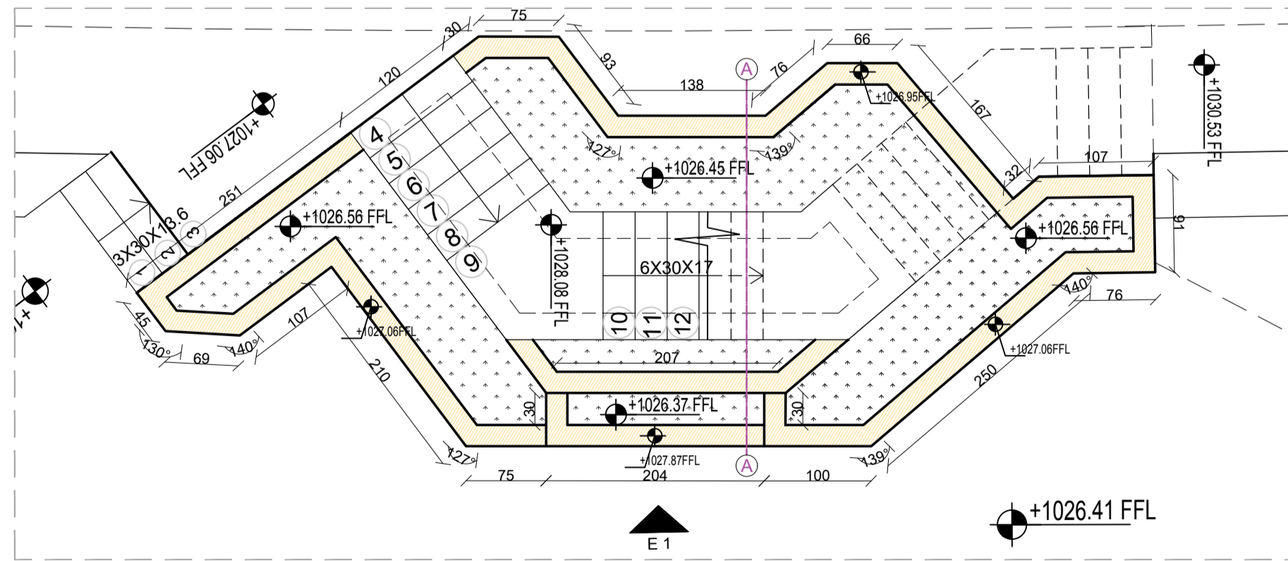
STAIRS 05-PLAN VIEW SCALE:1-50
